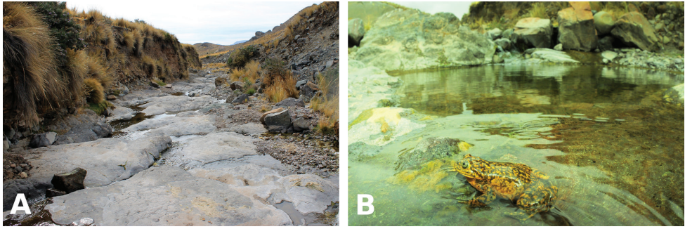
Figure 5. Habitat of T. ventriflavum at the type locality (A) and detail of stream pool used by adults and tadpoles (B). Photographs by V. Vargas García (A) and A. Catenazzi (B).
