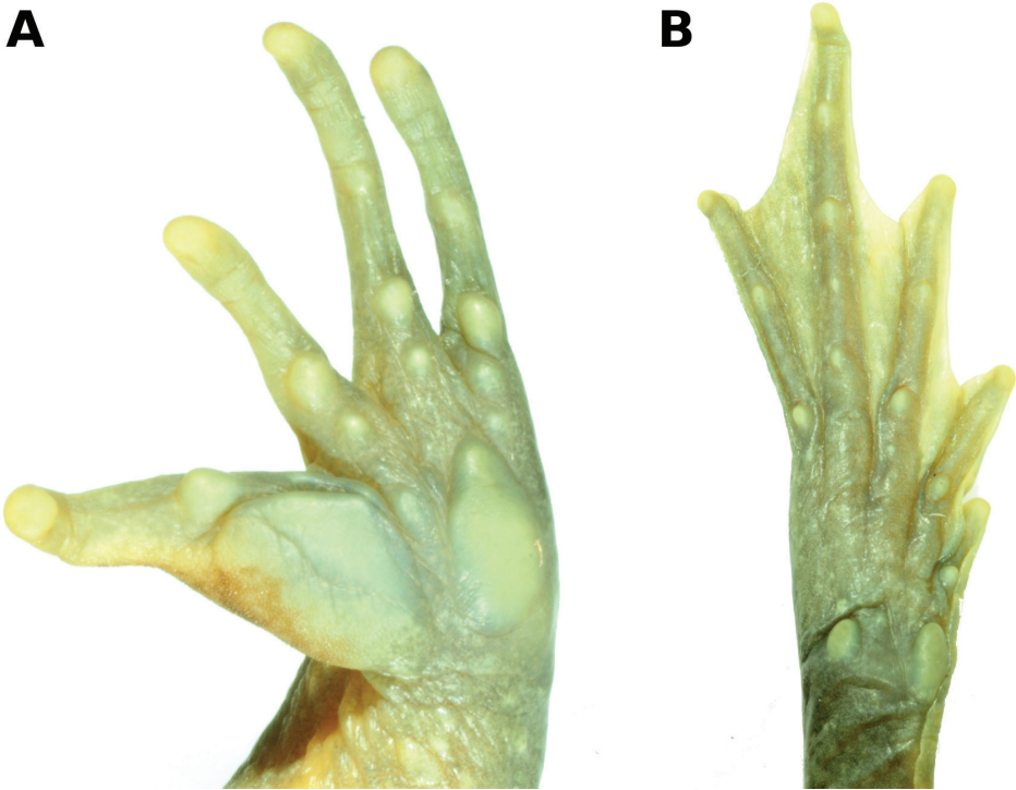
Figure 4. Ventral views of hand ( A ) and foot ( B ) of Telmatobius ventriflavum sp. n. (holotype, CORBIDI 14685, SVL 48.5 mm). Photographs by A. Catenazzi.
