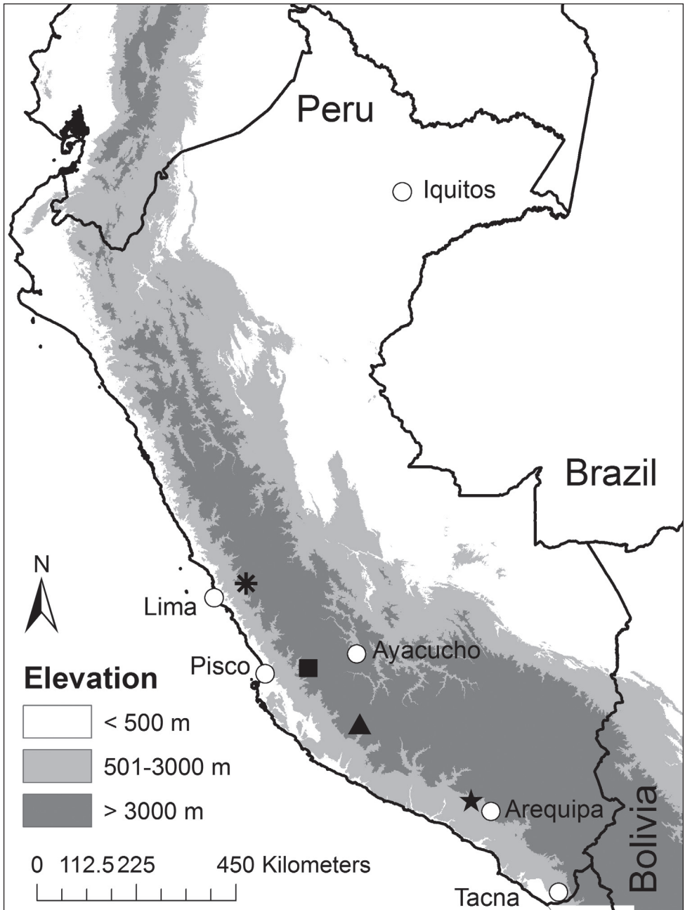
Figure 1. Map of Peru indicating the type localities of Telmatobius ventriflavum sp. n. (square), T. rimac (asterisk), T. intermedius (triangle) and T. arequipensis (star). The type locality of T. peruvianus is presumed to be near Tacna.
