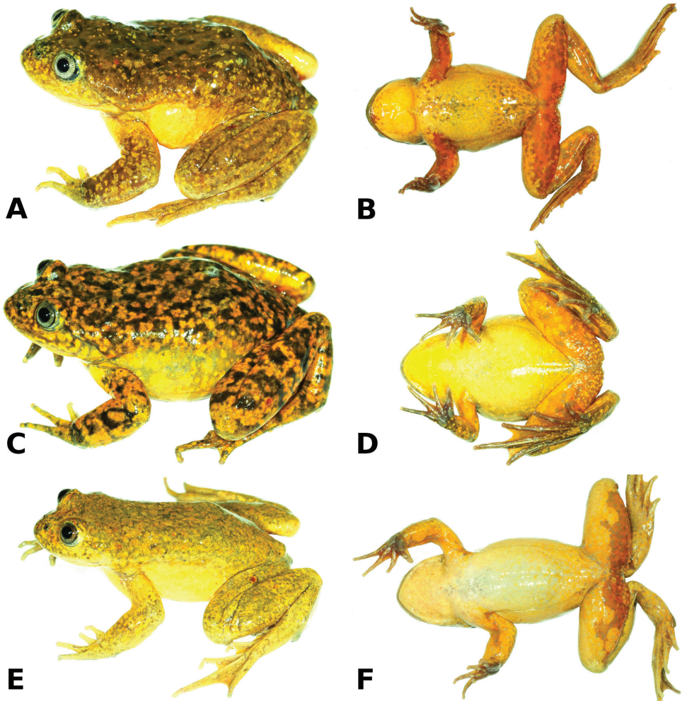
Figure 2. Live holotype of Telmatobius ventriflavum sp. n., male CORBIDI 14685 (SVL 48.5 mm) in dorsolateral (A) and ventral (B) views. Live paratypes, female CORBIDI 14684 (SVL 52.9 mm; C, D), and female CORBIDI 14686 (SVL 51.5 mm; E, F) in dorsolateral and ventral views. Photographs by A. Catenazzi.
