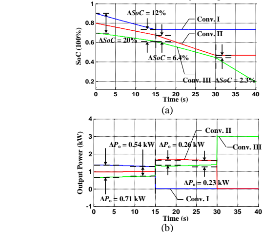
Fig. 15. Discharging process with dynamic disconnection of ESUs.
