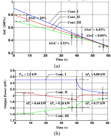
Fig. 19. Effect of saturation limiter in the discharging process.
