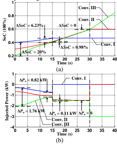
Fig. 14. Charging process with dynamic disconnection of ESUs.
