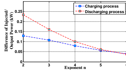
Fig. 17. Final errors of injected/output power with different exponent n.
