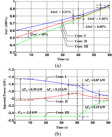
Fig. 18. Effect of saturation limiter in the charging process.
