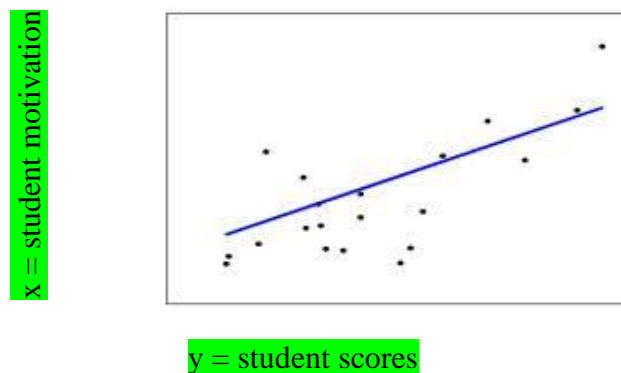
Figure 1: Linear Regression Representation
