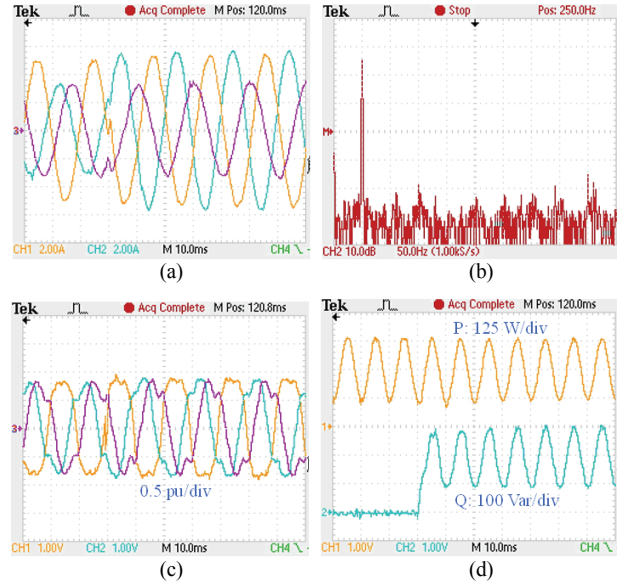
Fig. 4. Experimental results of sinusoidal current control. (a) grid current (b) current harmonic spectrum, (c) modulation waveform, (d) inverter power
