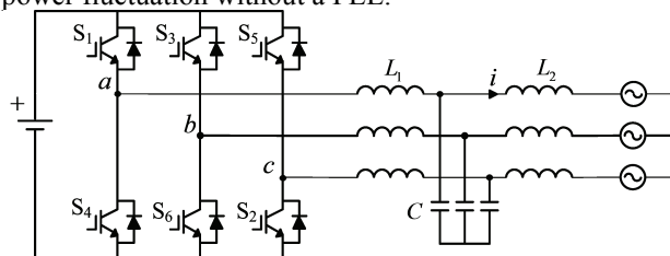
Fig. 1. Schematic diagram of grid-connected inverter
