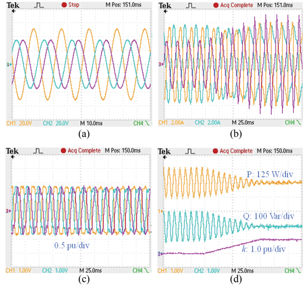
Fig. 5. Experimental results of proposed method under unbalanced conditions. (a) grid voltage, (b) grid current, (c) inverter modulation waveform, (d) inverter output power
