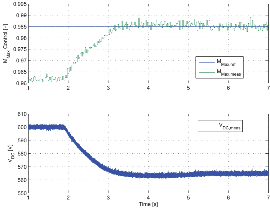
Figure 7: Experimental operation of the M_{Max} controller
