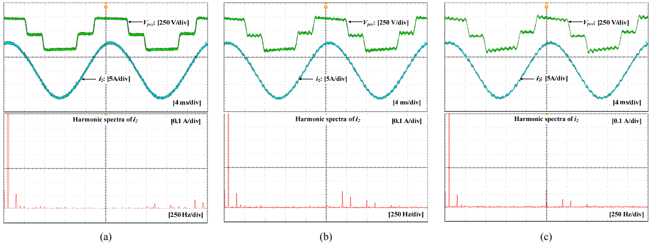
Fig. 18. Measured A-phase PCC voltage and grid current with the high cut-off frequency of high-pass filter ( \omega_c=3\omega_s ) for harmonic compensation. (a) L_g=0 mH. (b) L_g=4.5 mH. (c) L_g=9 mH.
