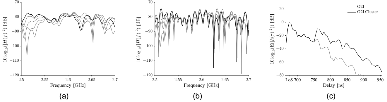
Fig. 2. Transfer functions corresponding to five array elements with \lambda/10 spacing (in x -direction) are given for the outdoor-to-indoor channel without outdoor scatterer (a) and with one outdoor scatterer (b). The averaged squared magnitude of the related impulse responses obtained for a Hann pulse with 200 MHz bandwidth are depicted in (c).
