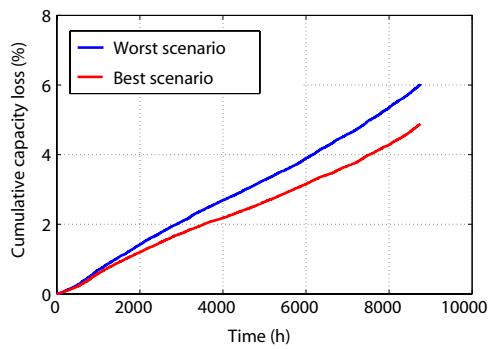
Fig. 13. Annual cumulative loss of VRLA battery capacity.
