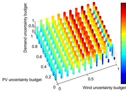
Fig. 8. Wind capacity (kW) in case of Li-Ion batteries for different budgets of uncertainty.
