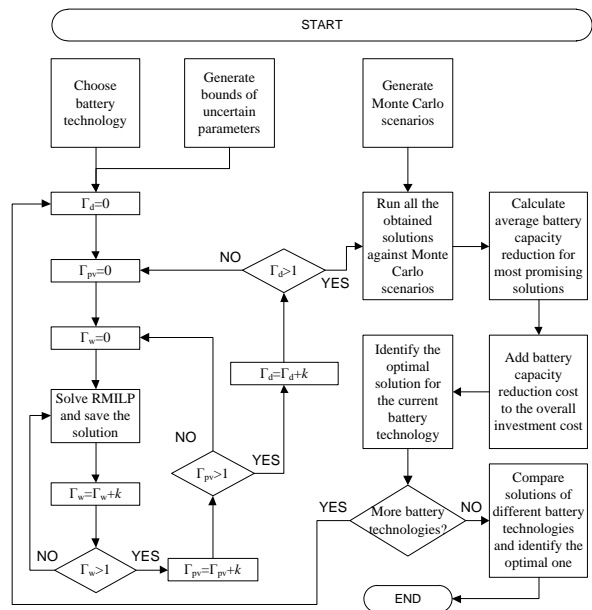
Fig. 2. Solution algorithm.
