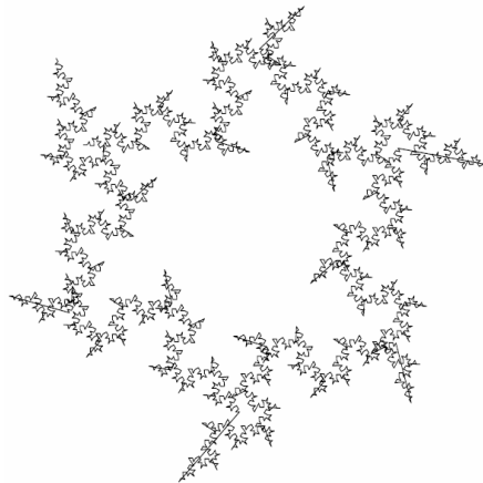
Figure 2 The Koch curve with random element added to the iterative step
