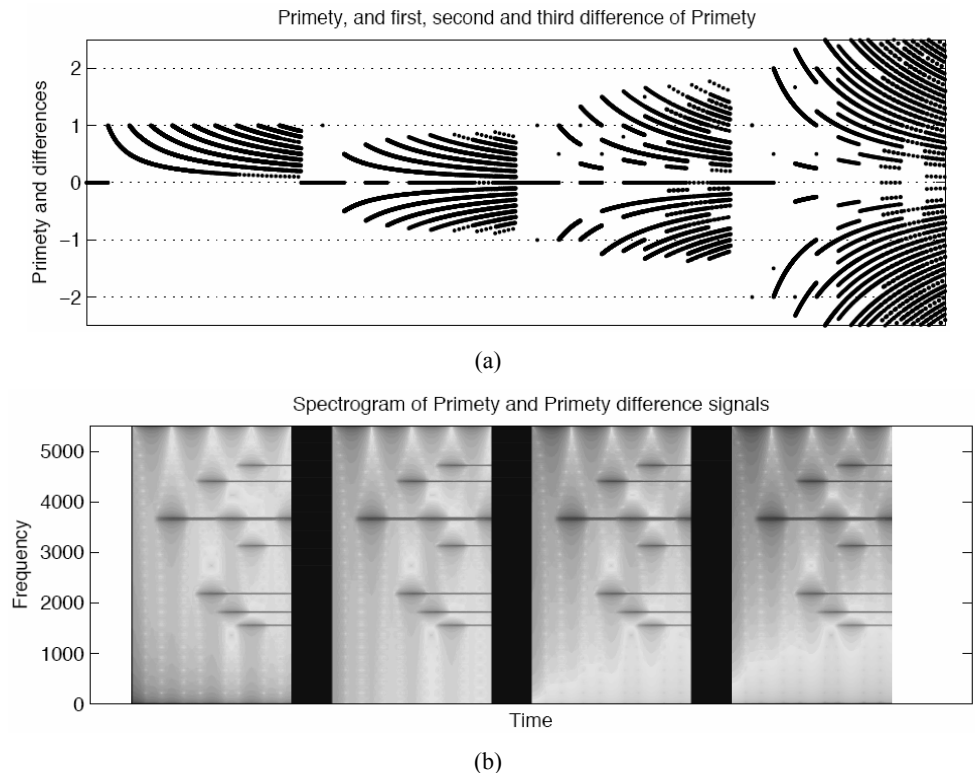
Figure 12 (a) Real value primety function and first three difference signals, and (b) spectrograms
