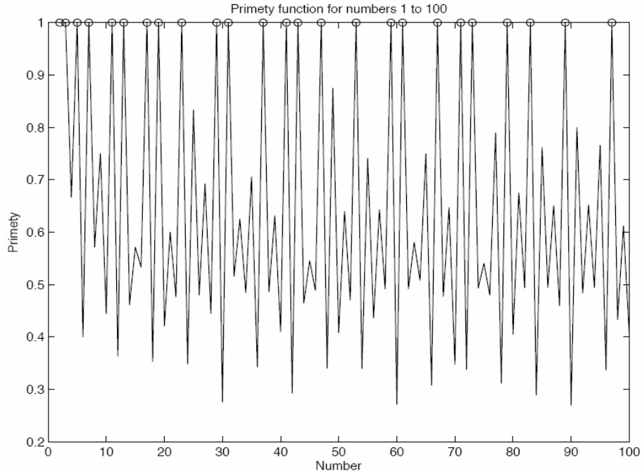
Figure 7 The primety values for real numbers between 1 and 100
