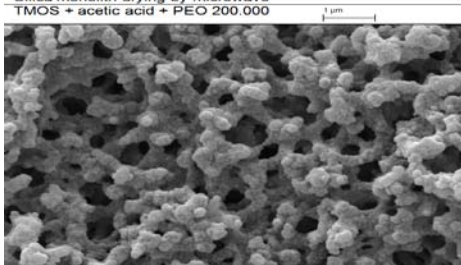
Silica monolith drying by microwave TMOS + acetic acid + PEO 200.000
