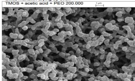
Silica monolith drying by oven TMOS + acetic acid + PEO 200.000
