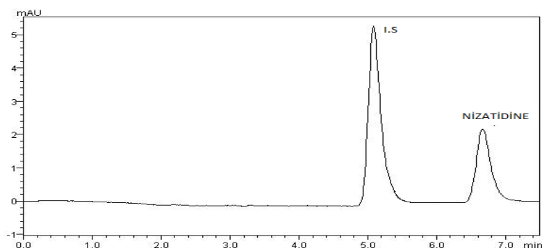
Figure 1. Chromatograms obtained from standards mixtures: Chromatogram of standard mixture; Nizatidine (1 µg/mL) and Internal standard (2 µg/mL)
