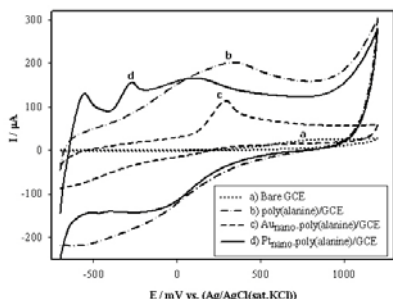
Fig.1 Cyclic voltammograms of 1.0 mM hydrazine oxidation in 0.1 M pH 7.0 phosphate buffer solution at different modified electrodes. Scan rate 50 mV/s.
