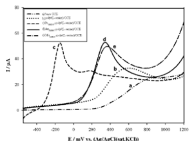
Fig. 1 Linear sweep voltammograms of 1.0 mM hydrazine oxidation in 0.1 M pH 7.0 phosphate buffer solution at different modified electrodes. Scan rate 50 mV/s
