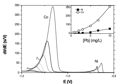
Fig.1. CC-AdSCP curves recorded for increasing concentrations of Pb in the solution of 5 \cdot 10^{-9} M Co, 5 \cdot 10^{-8} M Ni, 0.1 M ammonia buffer, 5 \cdot 10^{-5} M nioxime, 0.25 M \text{NaNO}_2 at the PbFE in situ . Preconcentration: -1.45 V for 20 s, accumulation: -0.75 V for 60 s; stripping current: 2 \mu\text{A} .
