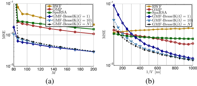
Fig. 6. Comparison of the MSE achieved by the different algorithms versus (a) number of pilot symbols M and (b) cluster rate 1/V . In (a) the channel parameters are 1/V = 300 ns, 1/v = 5 ns, U = 60 ns, and u = 20 ns. In (b) M = 100 , and we have 1/v = 5 ns, U = 900 ns, and u = 20 ns.
