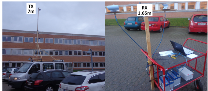
Fig. 1: Transmitter and receiver setup.
