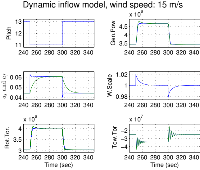
Fig. 4. Simulation for wind speed 15 m/s and average pitch at 12 deg. Otherwise similar to figure 3.
