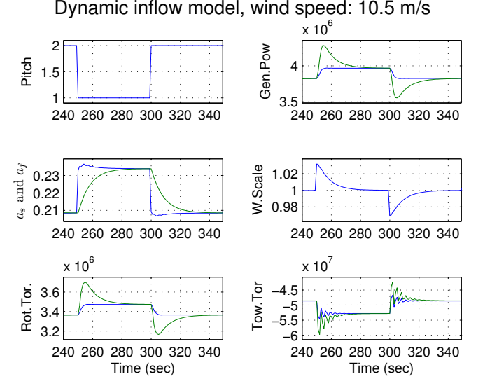
Fig. 3. Simulation close to rated wind speed with constant wind and stepping pitch angle. In the plots the blue line is without dynamic inflow and the green is with dynamic inflow except in the plot of induction factors where blue is the static and green is the filtered induction factor. W.Scale is the wind scaling factor in (16e), Rot.Tor is the rotor torque and Tow.Tor is the tower tilting torque.
