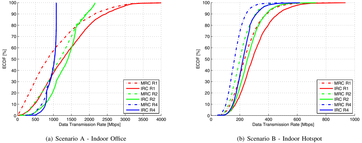
Fig. 2. ECDFs showing the data transmission rates in Mbps for both detector types (MMSE-MRC and MMSE-IRC) and different frequency reuse schemes.
