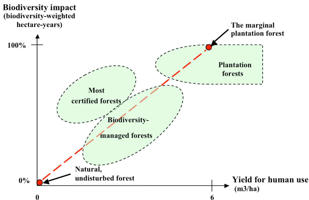
Figure 1: The place of different forest management systems (dashed green ovals) relative to the iso-biodiversity line (dashed red line), its determining extremes (red dots).
