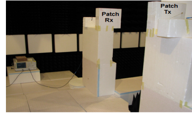
Fig. 3. Measurement setup in the anechoic chamber.
