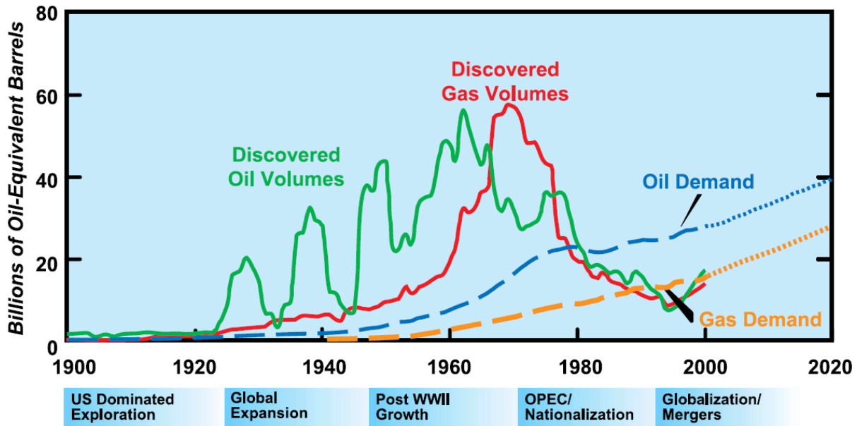
Figure 12: Historical discovery and consumption of fossil fuel [12].
