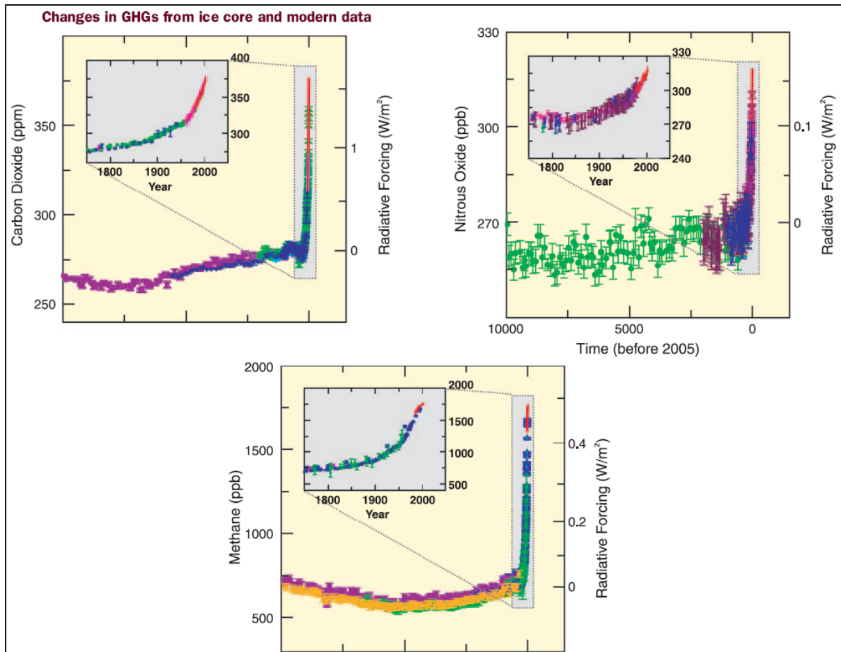
Figure 3: Concentration of CO 2 , CH 4 , and N 2 O in the earth's atmosphere over the last 10,000 years [4].
