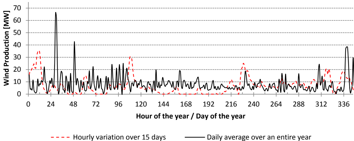
Figure 3: Wind power production the first 15 days of the year in Jordan. Based on WindPRO[54] analyses using MERRA data.
