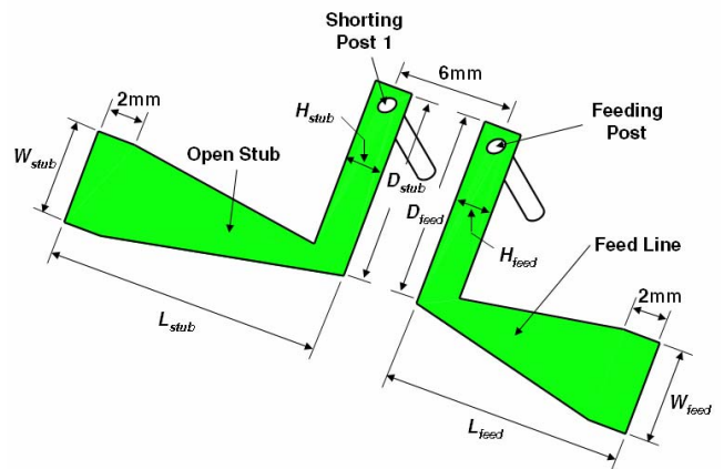
(b) Feed line and open stub ( D_{shorting}=18\text{mm} , H_{feed} , H_{stub}=2\text{mm} , D_{feed} , D_{stub}=10\text{mm} , W_{feed}=4\text{mm} , L_{feed}=12\text{mm} , W_{stub}=6\text{mm} and L_{stub}=14\text{mm} ).
