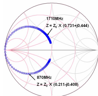
(b) BRF (LC series resonator) parallel to load.
