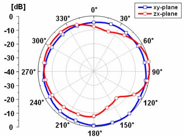
(c) Radiation pattern at 1795MHz
