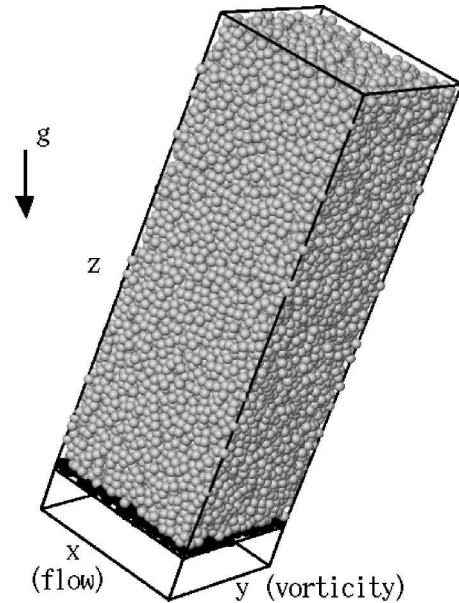
FIG. 1. Typical 3D snapshot for chute flow: N=24,000 , with bottom surface dimensions 20 \times 20 diameters shown by the black particles fixed to the bottom plate; tilt angle \theta=24^\circ , coefficient of restitution \epsilon=0.88 , and friction coefficient \mu=0.50 . Flow is directed down the incline.
