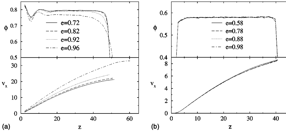
FIG. 10. Density and velocity profiles for different values of \epsilon for (a) Model L2 at \theta=20^\circ, H=50 for \epsilon=0.72, 0.82, 0.92 , and 0.96 , and (b) Model L3 at \theta=22^\circ, H=40 for \epsilon=0.58, 0.78, 0.88 , and 0.98 .
