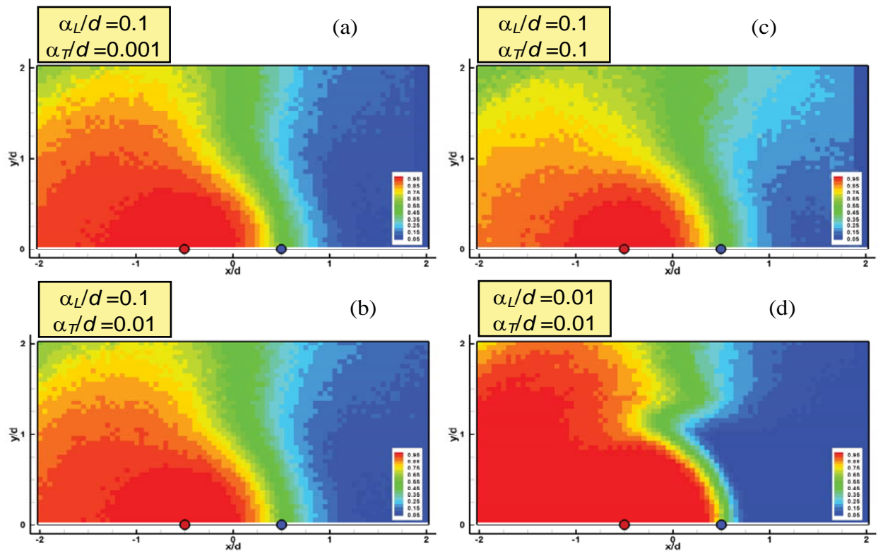
Figure 8. Impact of dispersivities on transient capture zones ( Qt_c/(md^2\phi)=8.64 ; t_c a/d^2=86.4 ).
