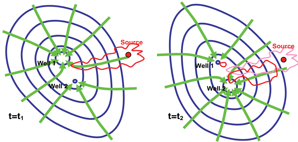
Figure 1. Schematic representation of the impact of flow transients on the contaminant plume. The contaminant source is within the capture zones of both wells but steady-state/advective-only capture zone analyses will give us an incorrect result.
