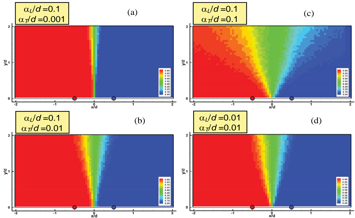
Figure 7. Impact of dispersivities on transient capture zones ( Qt_c/(md^2\phi)=0.0864 ; t_c a/d^2=86.4 ).
