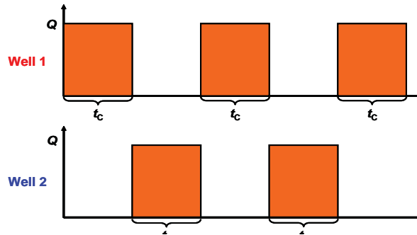
Figure 3. Temporal variability of pumping rates of Well 1 and 2.
