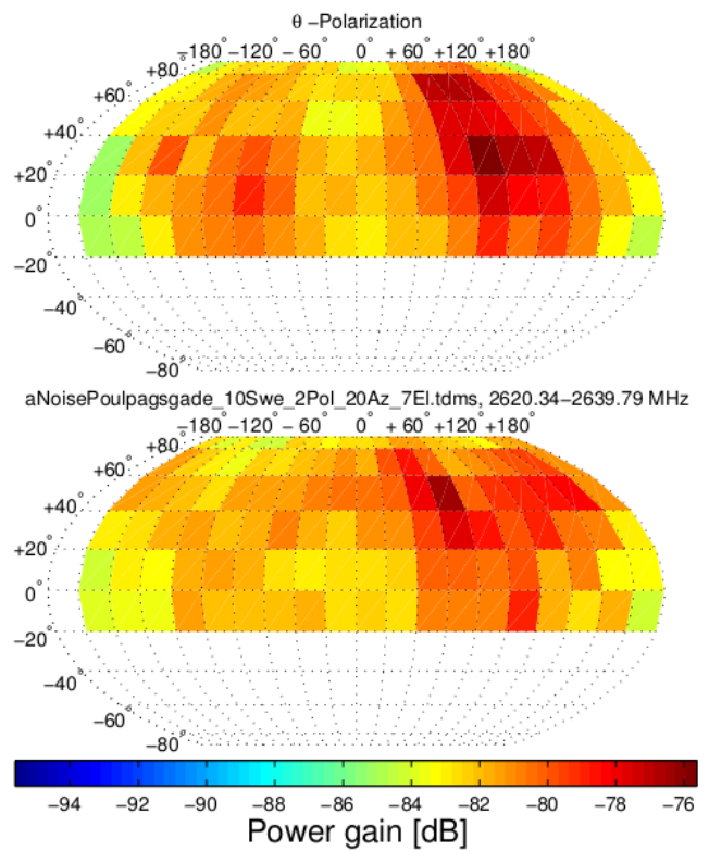
Fig. 9. Estimated power distribution for the LTE2500a1 band for the City measurement location.
