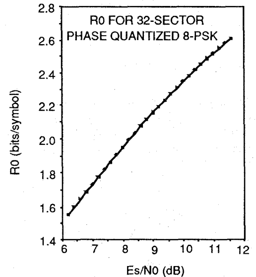
Fig. 5. R0 for 32-sector phase quantized 8-PSK with optimal spacing, and configuration of kind shown in Fig. 4.
