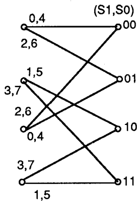
Fig. 3. 4-state 8-PSK Trellis Diagram.
