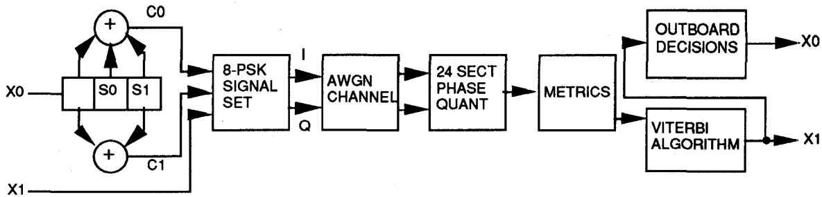
Fig. 1. 4-state 8-PSK system
