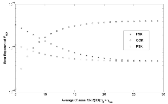
Fig. 3. Miss error exponents for counting rule with P_d = 0.3 and P_f = 0.001 .
