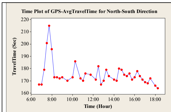
Figure 2- Time Plot of GPS Avg-Travel Time for North-South Direction
