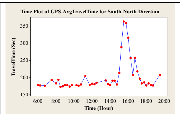
Figure 3- Time Plot of GPS Avg-Travel Time for South-North Direction
