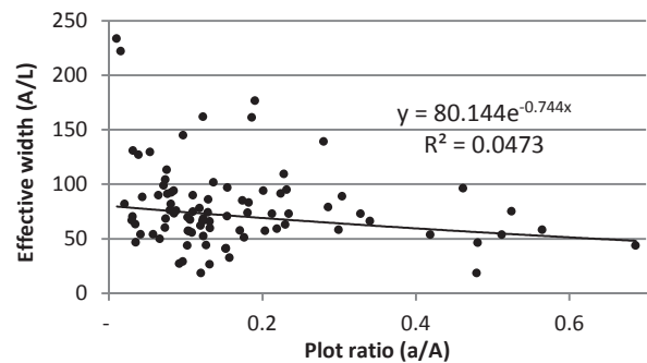
Figure 2: Effective width based on 88 DH areas in Aarhus
