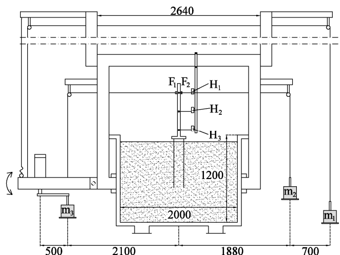
Fig. 1: Sketch of the test setup for cyclic loading with dimension in mm. F1 and F2 denote the force transducers and H_1 , H_2 and H_3 denote the horizontal displacement transducers. m_1 , m_2 and m_3 are the weights of mass.
