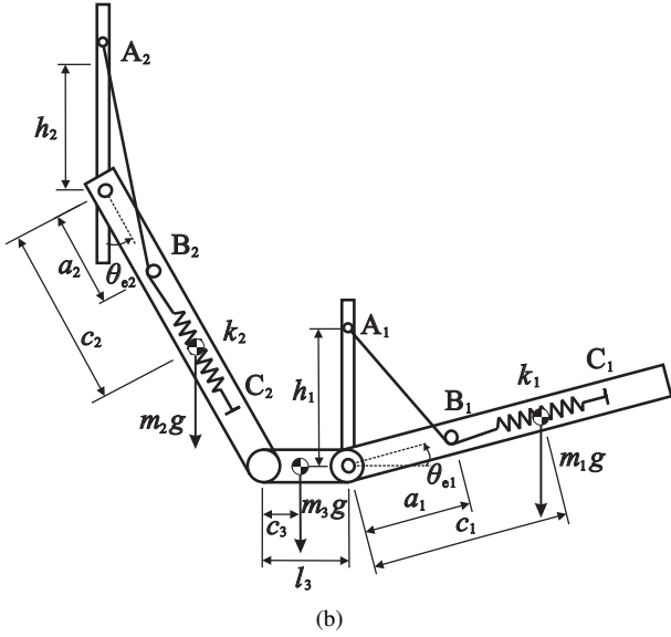
Fig. 1. Gravity compensation system of the exoskeleton, (a) parallel structure, (b) schematic diagram of the spring system.
