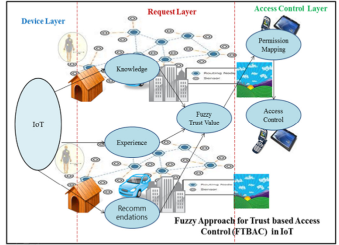
Figure.7: Proposed FTBAC Framework
