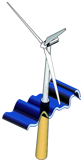
Figure 9.1: Sketch of a ballast stabilized floating wind turbine.
