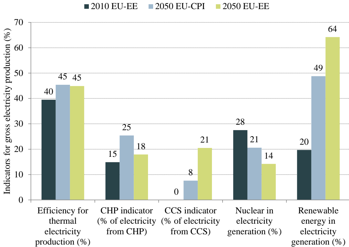
Figure 37: Indicators for gross electricity production in the EU-CPI scenario from the first pre-study [1] and the EU-EE scenario used in this study.
