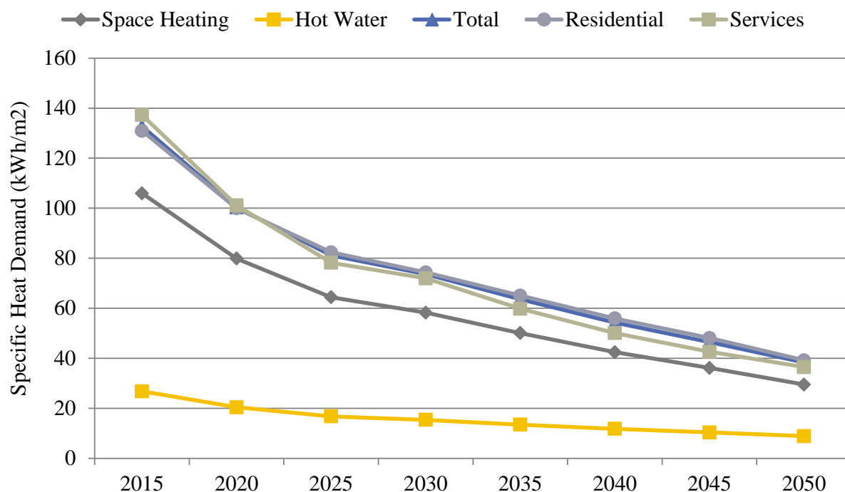
Figure 71: Specific heat demand in the Energy Efficiency scenario for the residential and non-residential/services sectors, as well as for the space heating, hot water, and total heat demand.
