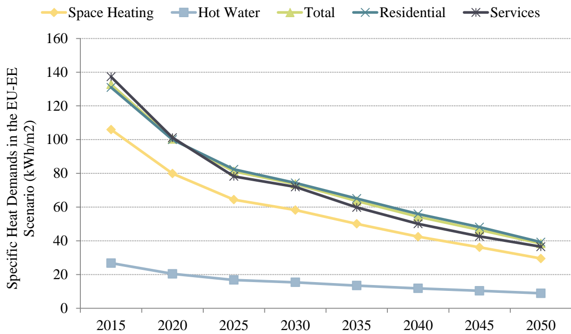
Figure 42: Specific heat demand in the EU-EE scenario for the residential and services sectors, as well as for the space heating, hot water, and total heat demand.
