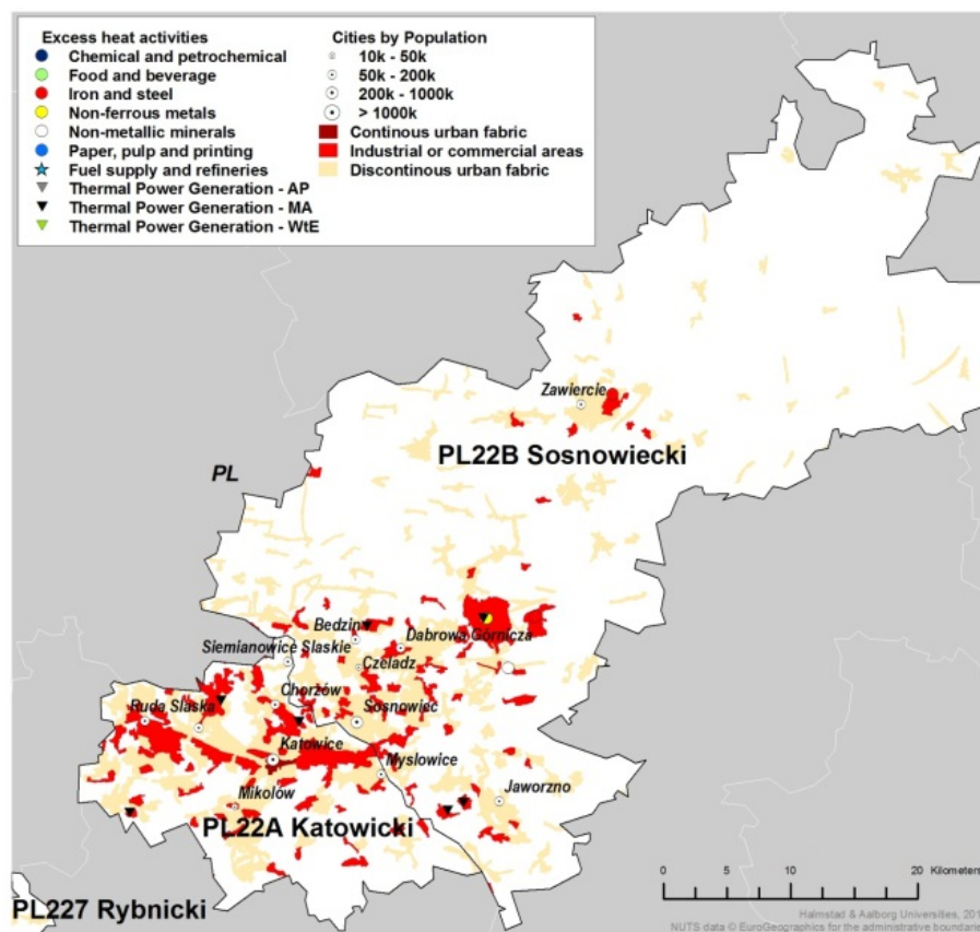
Figure 31: Example of Refurbishment NUTS3 region excess heat hot spots: PL22A Katowicki and PL22B Sosnowiecki in Southern Poland.
