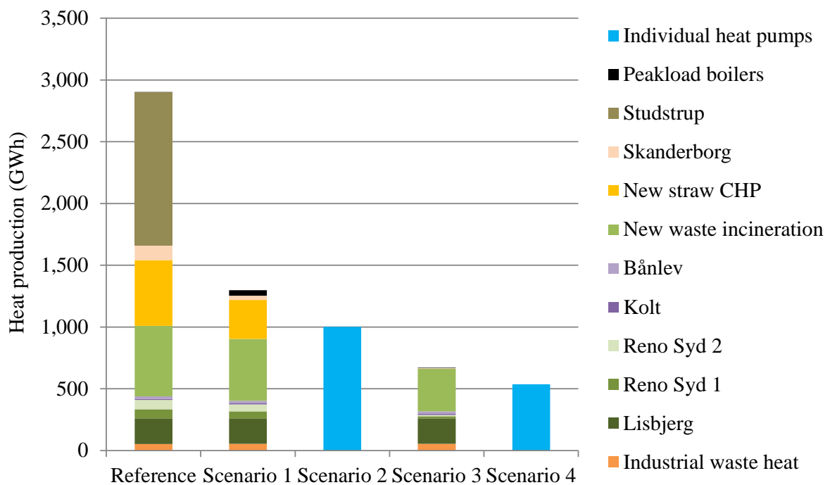
Figure 95: Annual heat production.
