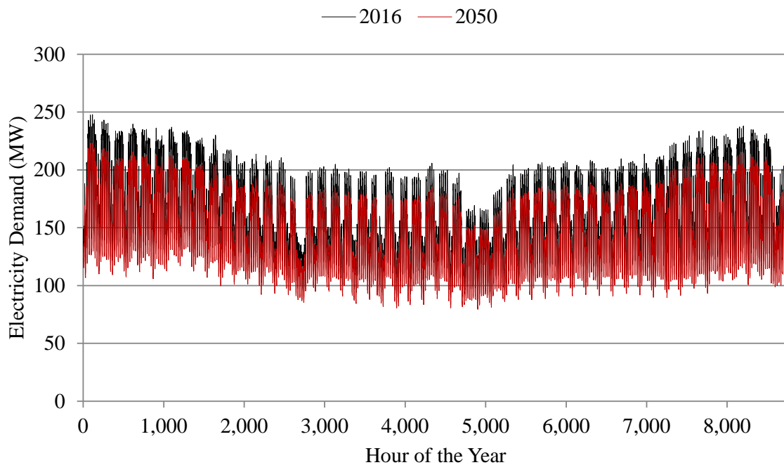
Figure 94: Hourly electricity load in the years 2016 and 2050.
