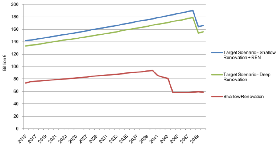
Figure 73: Investments for heating and ventilation systems per year EU27 [billion €/a]
