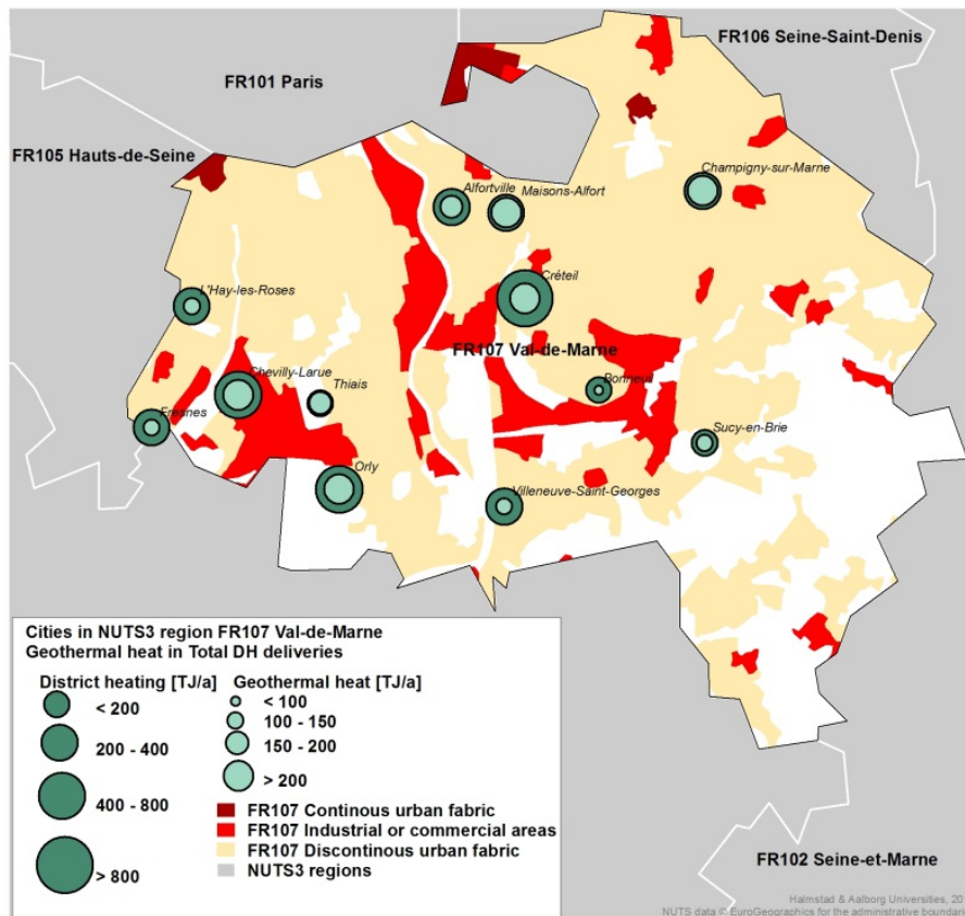
Figure 21: Cities with district heating and geothermal heat in French NUTS3 region FR107 Val-de-Marne [34].
