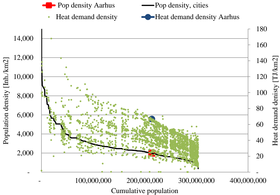
Figure 90: Population and heat demand density in European Cities based on [1].
