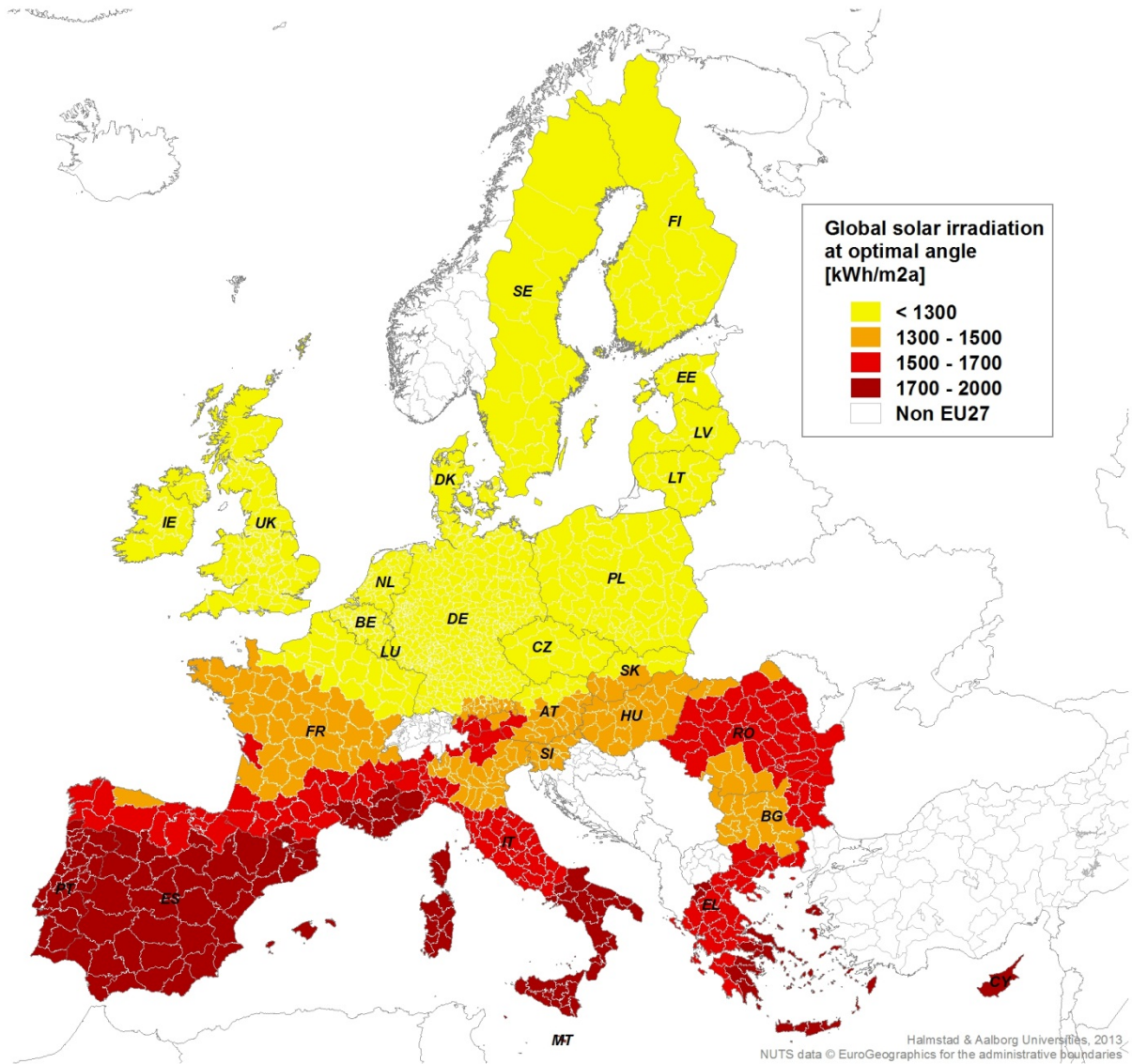
Figure 86: Annual solar irradiation on a south-oriented tilted surface at optimal angle by NUTS3 region.
