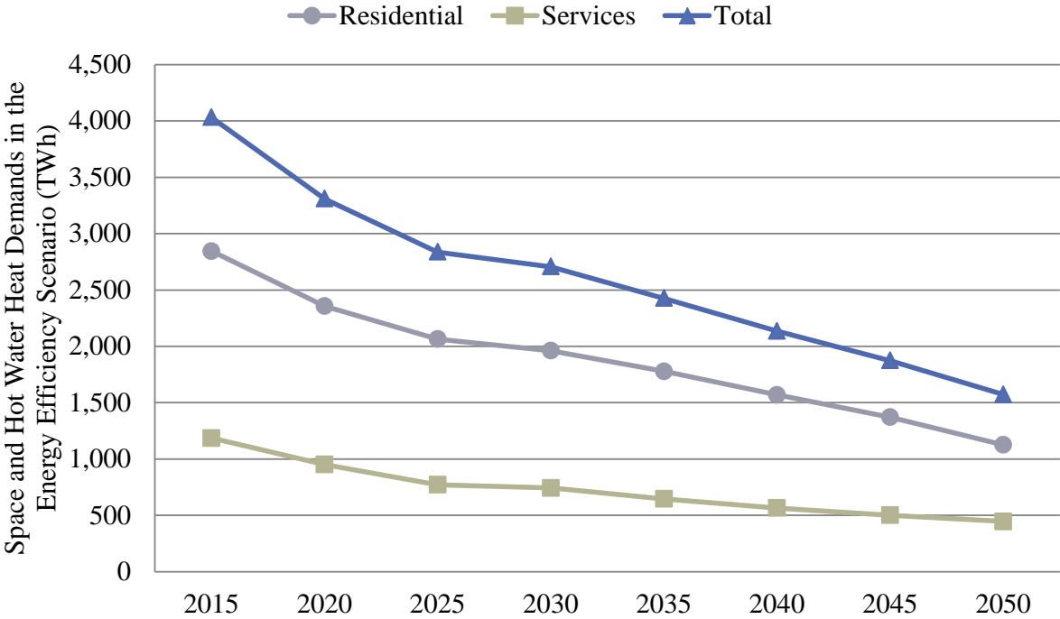
Figure 70: Residential and services heat demand in the Energy Efficiency scenario between 2015 and 2050.
