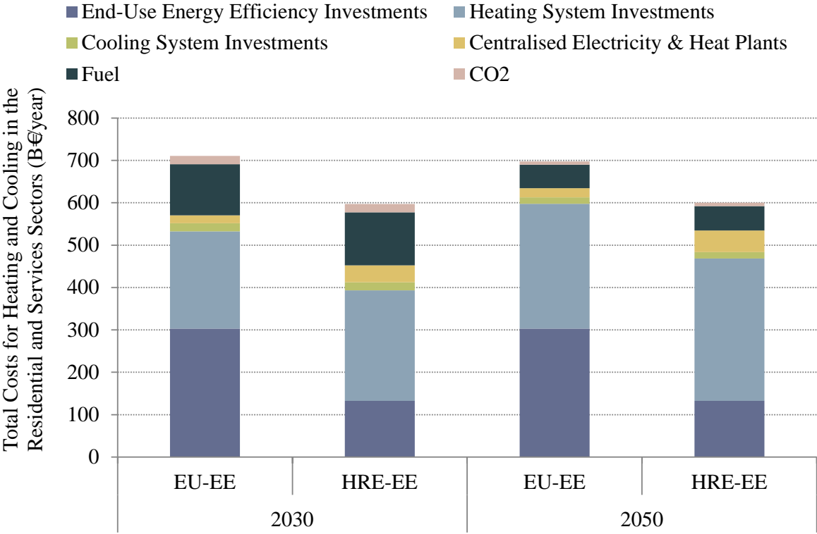
Figure 4: Total annual costs for heating and cooling in the residential and services sectors for the Energy Efficiency (EU-EE) and Heat Roadmap Europe 2 (HRE-EE) scenarios in the years 2030 and 2050.
