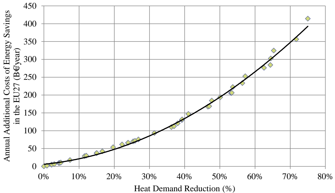
Figure 50: Annual ‘additional’ costs for energy efficiency measures that reduce the heat demand by different percentages based on Danish buildings (scenario C) [43], an interest rate of 3%, and assuming an average lifetime of 30 years. These are indicative only as they not consider the change in specific heat demand, but instead it considers the change in total heat demand.
