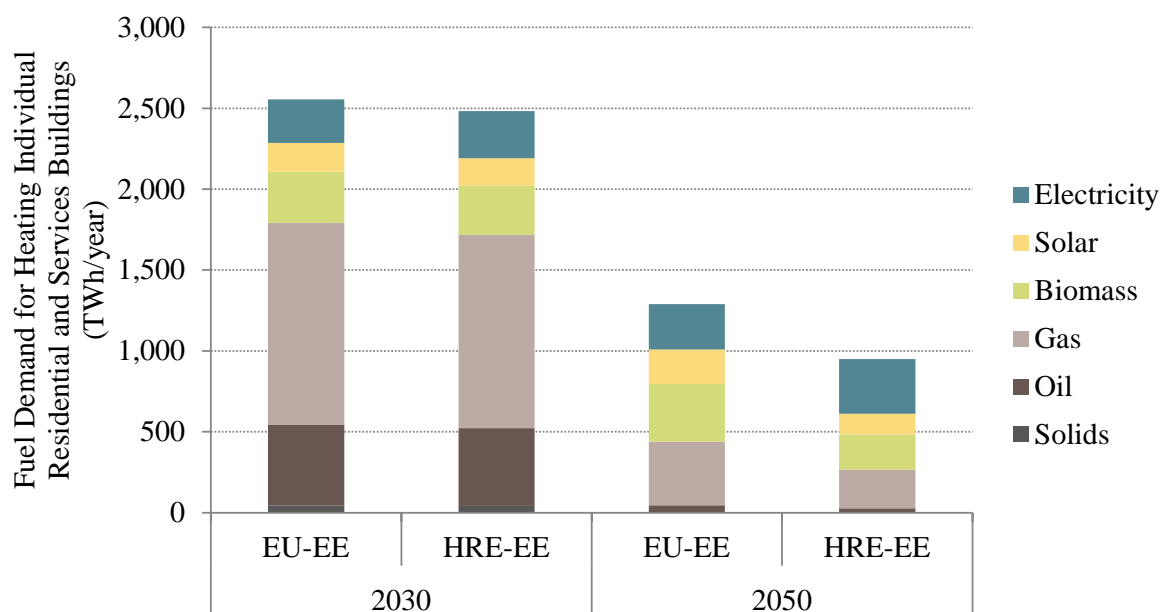
Figure 51: Fuel consumption by individual boilers in the EU-EE and HRE-EE scenarios for the years 2030 and 2050.
