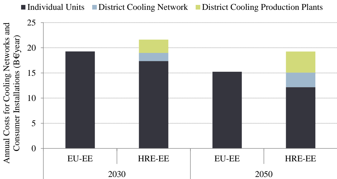
Figure 55: Annual cooling system costs for the EU-EE and HRE-EE scenarios for the years 2030 and 2050.
