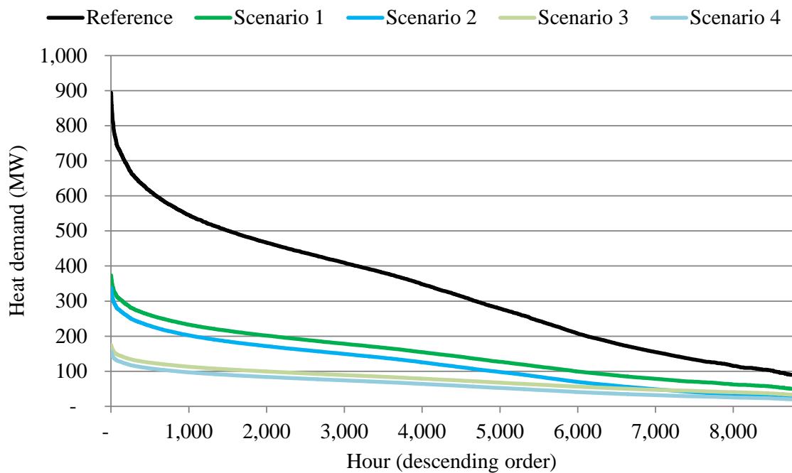
Figure 93: Hourly heat loads for the reference and both scenarios.
