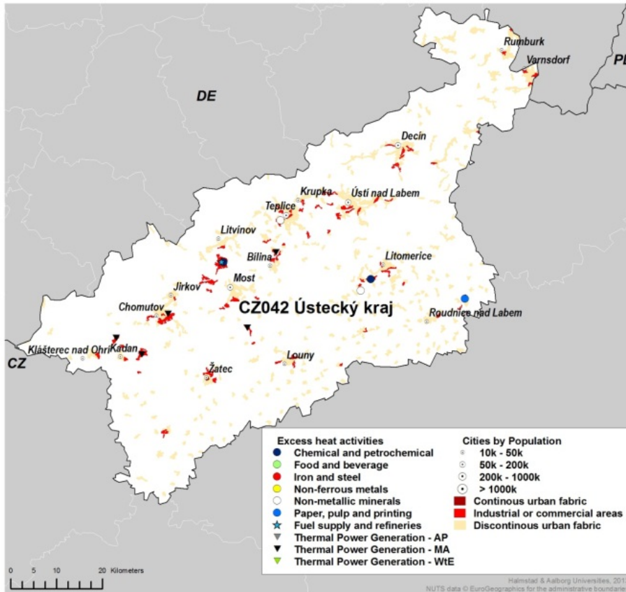
Figure 32: Example of Refurbishment NUTS3 region excess heat hot spots: Czech Republic NUTS3 region of CZ042 Ústecký kraj.
