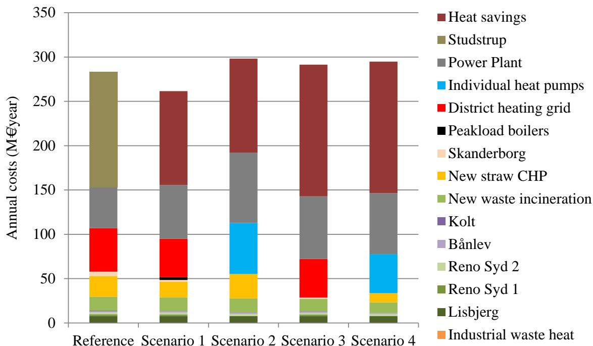
Figure 98: Annualised costs for all scenarios categorised by type of cost
