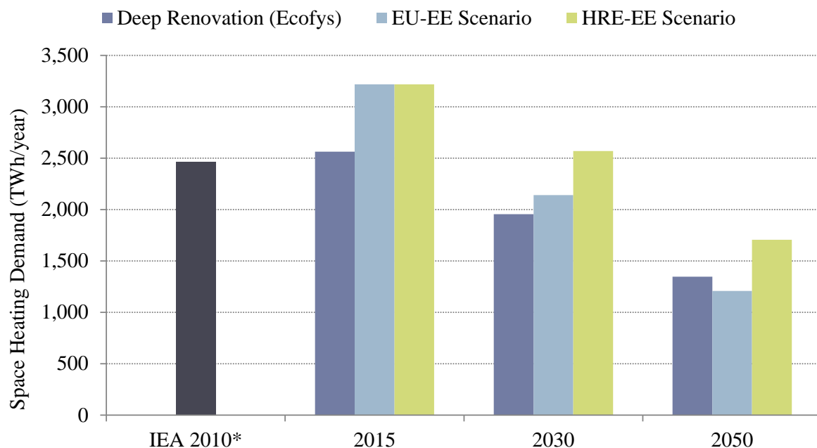
Figure 47: Space heating in the EU-EE scenario from the Energy Roadmap 2050 report [9], the Deep Renovation scenario from Ecofys [42], and the new space heating demand assumed in the HRE-EE scenario. *This space heating demand is estimated based on the total heat demand from the 2010 EU27 IEA Energy Balance minus the hot water demand identified from the PRIMES data for 2015.
