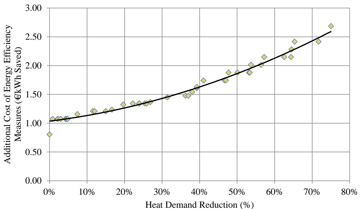
Figure 49: Additional costs for energy efficiency measures that reduce the heat demand by different percentages based on Danish buildings (scenario C) [43]. ‘Additional’ means it is assumed that these are the extra costs of completing the energy efficiency measures at the same time as implementing other building refurbishments.
