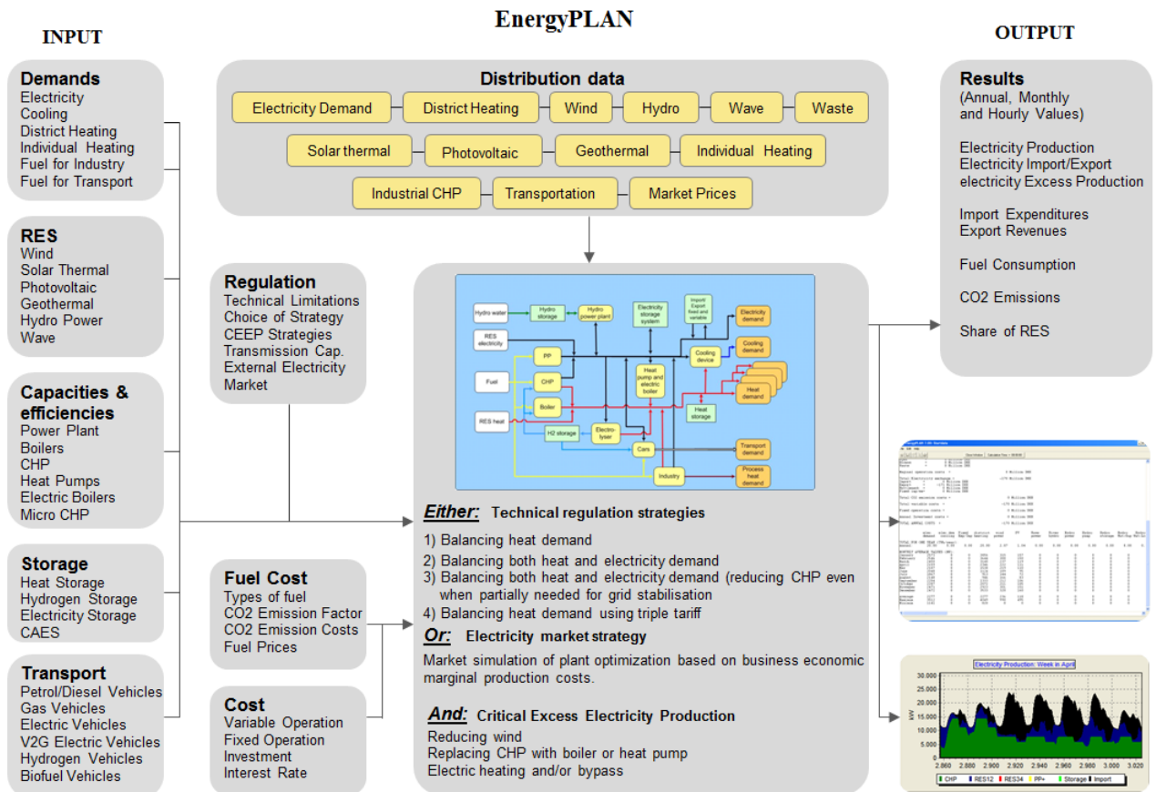
Figure 12: The structure of the EnergyPLAN tool [17].
