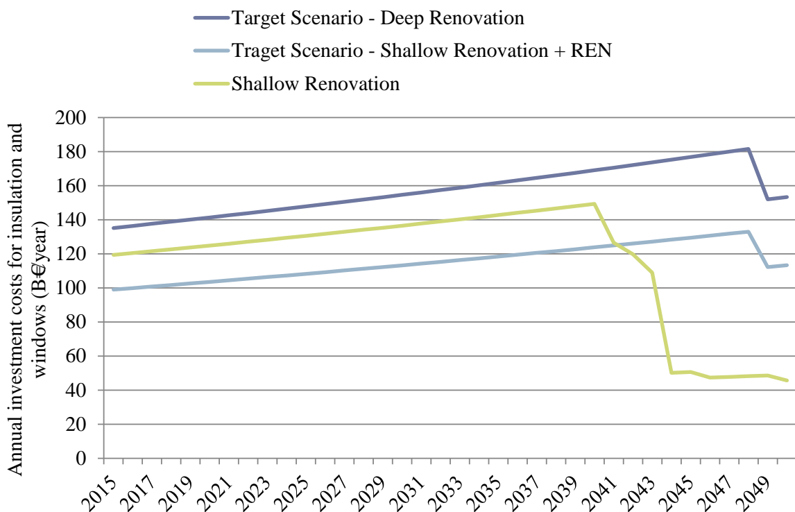
Figure 44: Annual investment costs for insulation and windows in the three scenarios created by Ecofys for energy efficiency in the EU27 [42].
