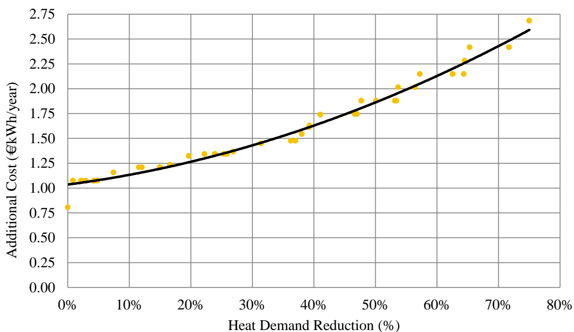
Figure 79: Additional costs for energy efficiency measures that reduce the heat demand by different percentages based on Danish buildings [Kragh,Wittchen, 2010].
