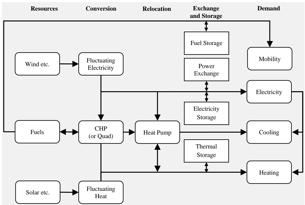
Figure 58: Interaction between sectors and technologies in a future sustainable energy system [52].
