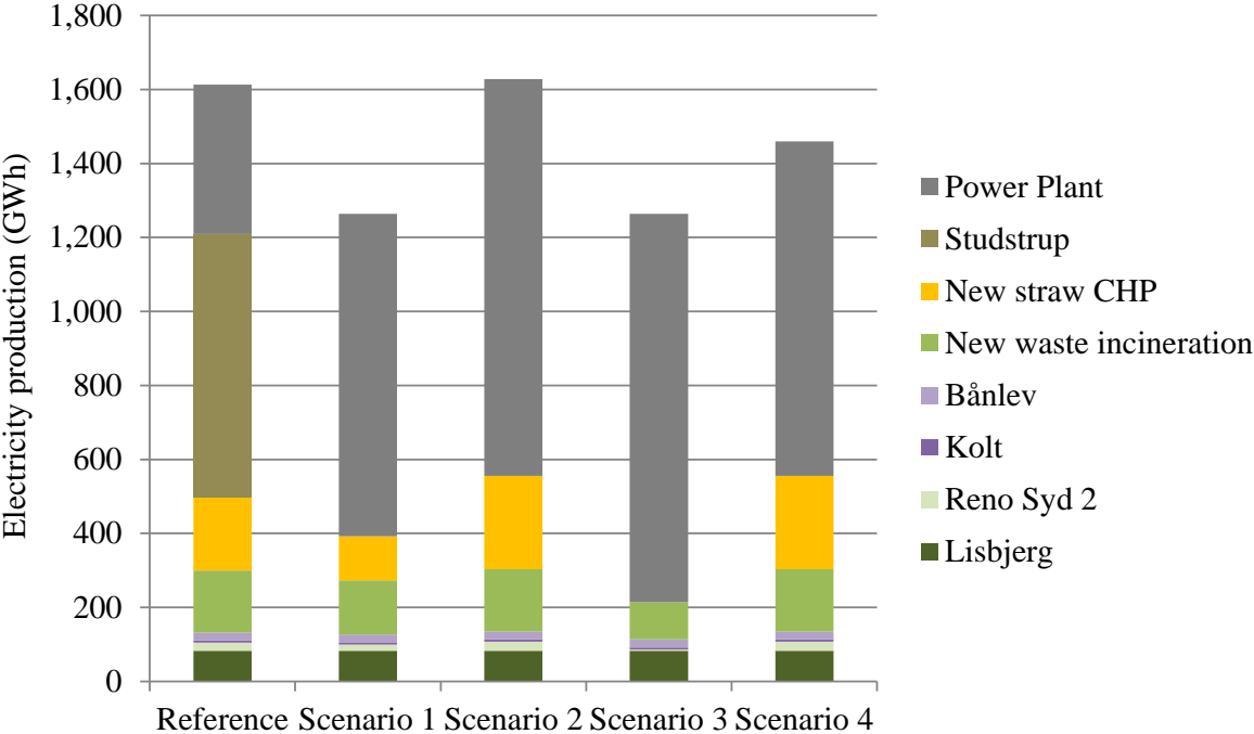
Figure 96: Annual electricity production.
