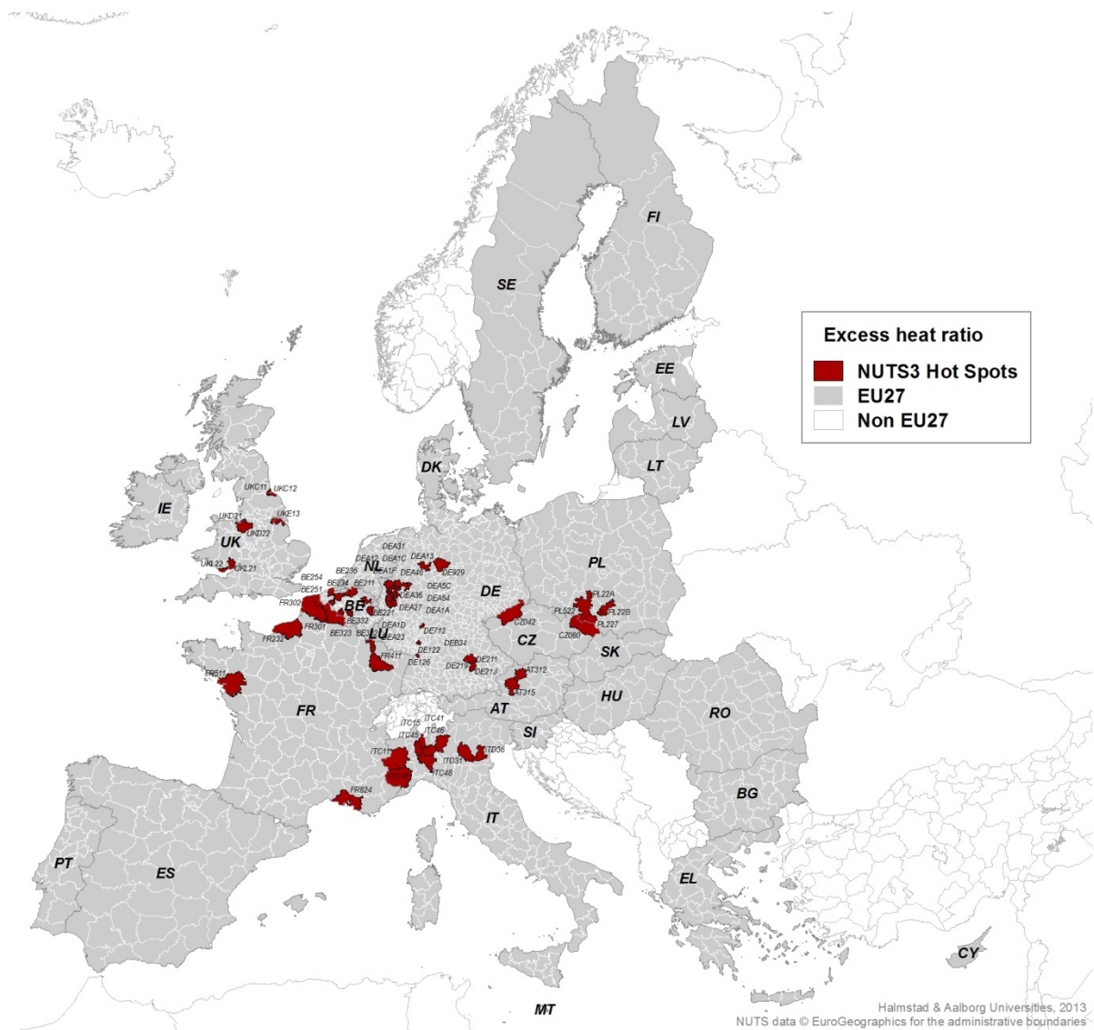
Figure 26: Selection of most promising EU27 NUTS3 region excess heat hot spots.
