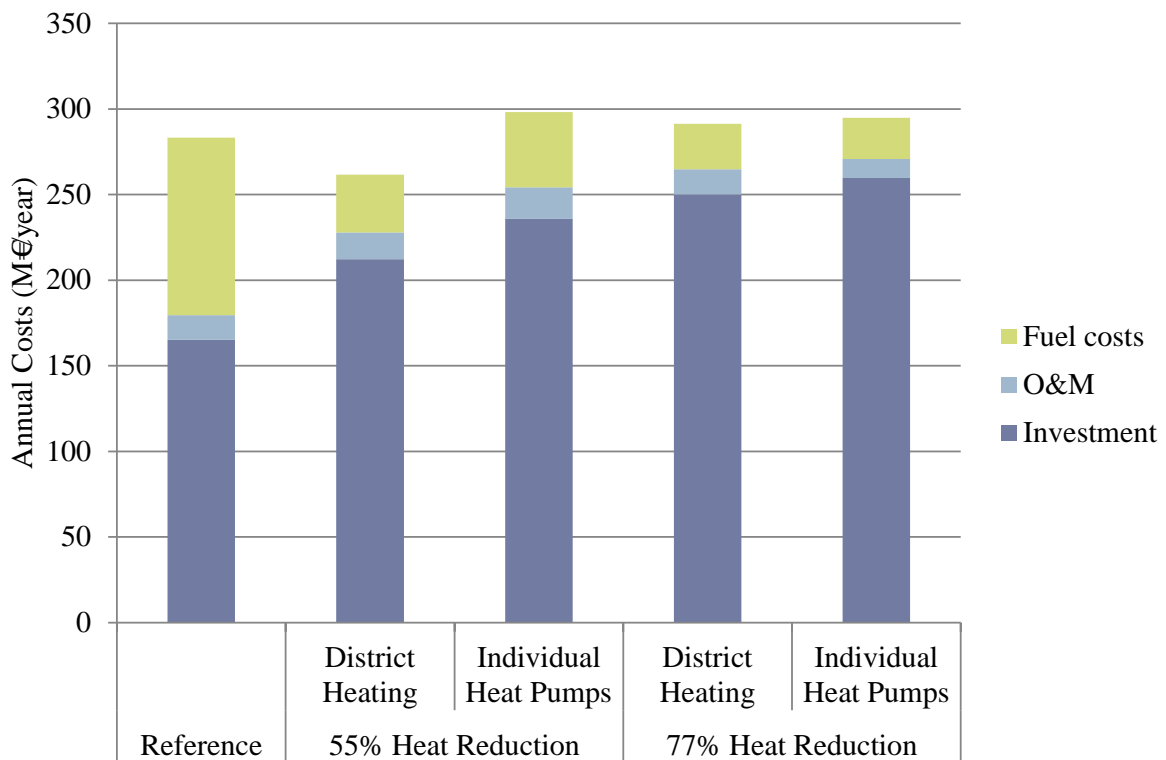
Figure 5: Annualised costs for all scenarios considered in the Aarhus case study.
