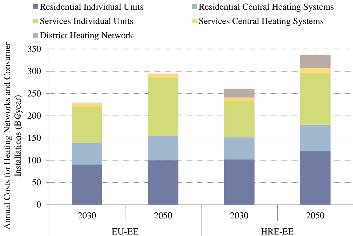
Figure 52: Annual investment and operation costs for heating networks and consumer installations for the EU-EE and HRE-EE scenarios in the years 2030 and 2050.
