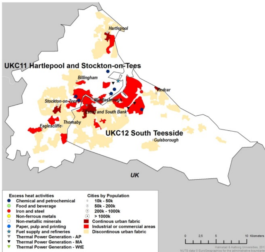
Figure 33: Examples of New Development NUTS3 region excess heat hot spots: twin United Kingdom NUTS3 regions of UKC12 South Teesside and UKC11 Hartlepool and Stockton-on-Tees.
