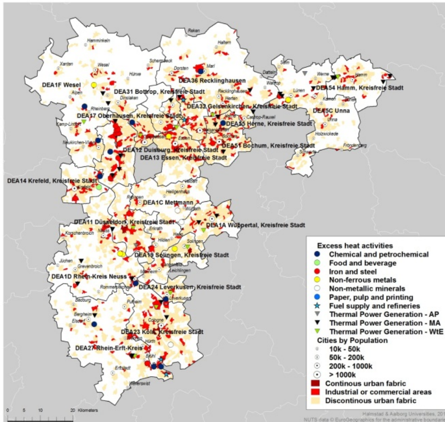
Figure 30: Example of Expansion NUTS3 region hot spots: large clusters of NUTS3 region excess heat hot spots in the Ruhr region of Germany.
