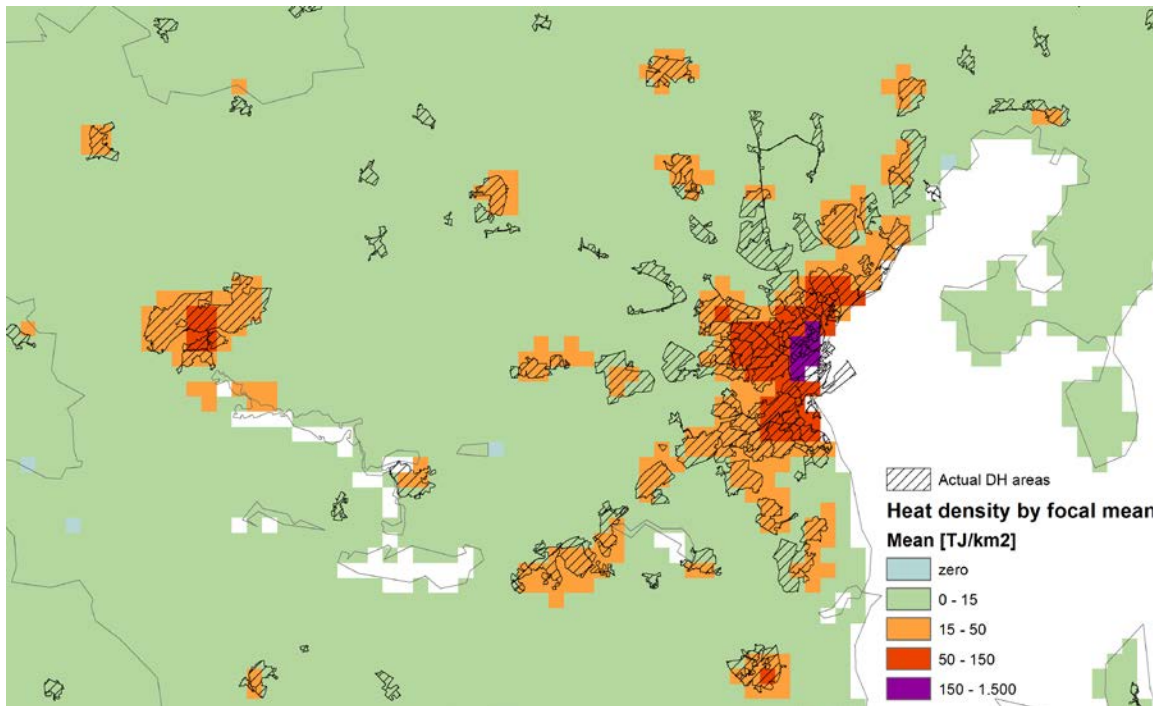
Figure 16: Comparison of prospective district heating areas found by the density method and existing district heating areas around the city of Aarhus, Denmark. The method can identify the majority of areas. The resolution of one square kilometre is just sufficient to identify all district heating areas above 10-20 TJ of annual heat demand.
