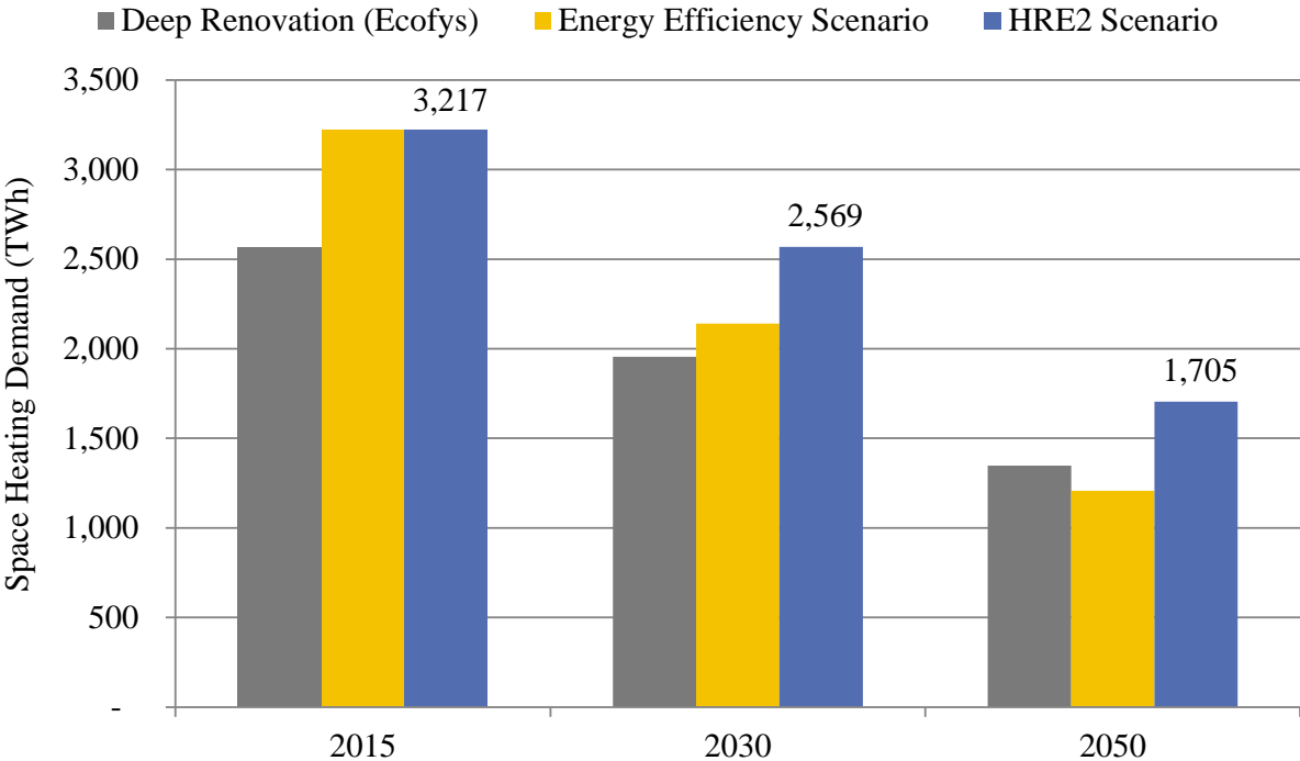
Figure 77: Space heating in the EE scenario from the Energy Roadmap 2050 [9], the Deep Renovation scenario from Ecofys [Boermans, Bettgenhäuser et al., 2012], and the new space heating demand assumed in this study.
