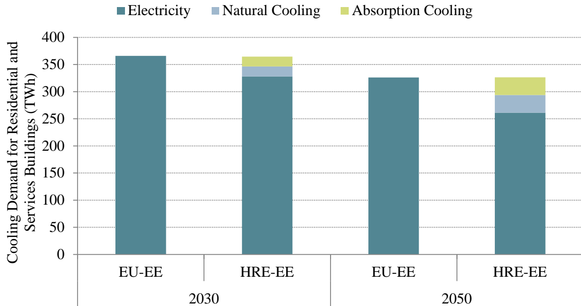
Figure 53: Cooling demand by fuel source for residential and services buildings in the EU-EE and HRE-EE scenarios for the years 2030 and 2050.
