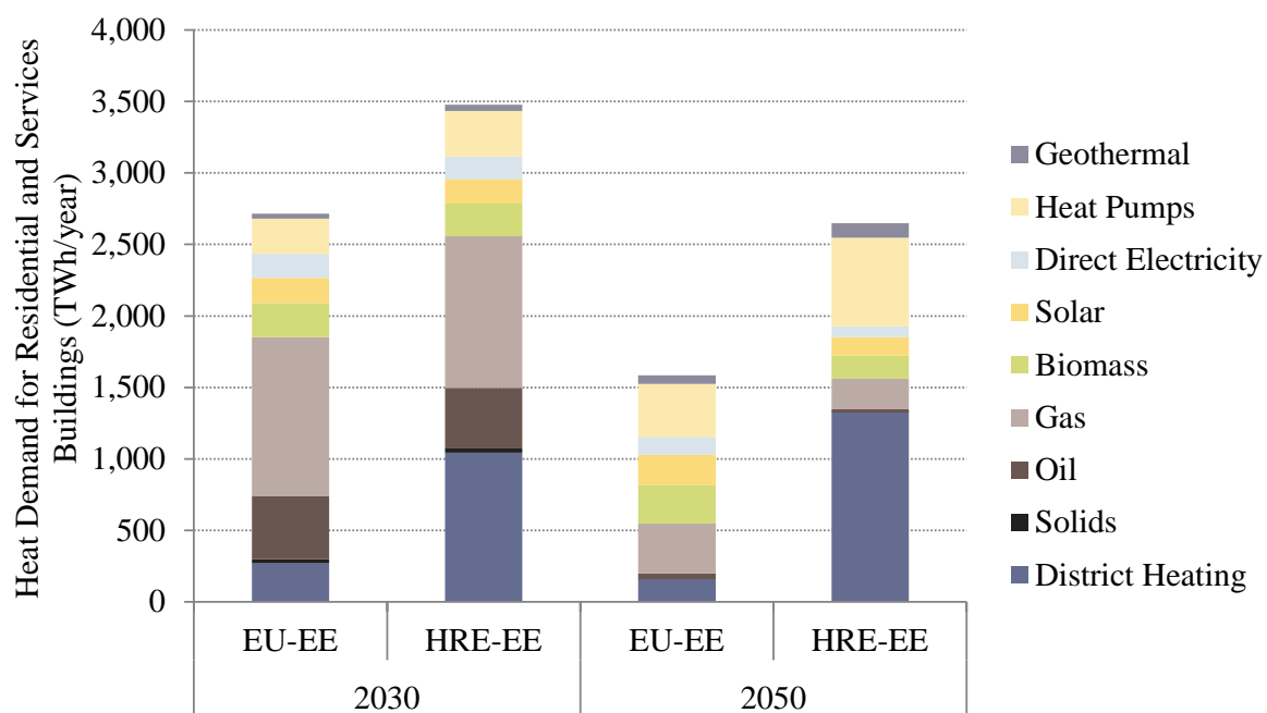
Figure 59: Heat demand by fuel for residential and services buildings in the EU-EE and HRE-EE scenarios for the years 2030 and 2050.
