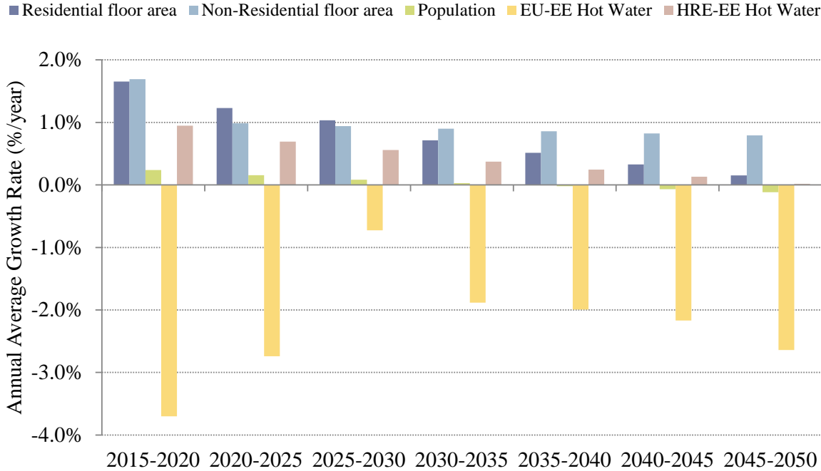
Figure 45: Average annual growth rates for the residential floor area, non-residential floor area, population, the original EU-EE scenario hot-water demand, and the new hot water demand assumed for the HRE-EE scenario (which is based on the average annual growth rate for the residential floor area and the population).
