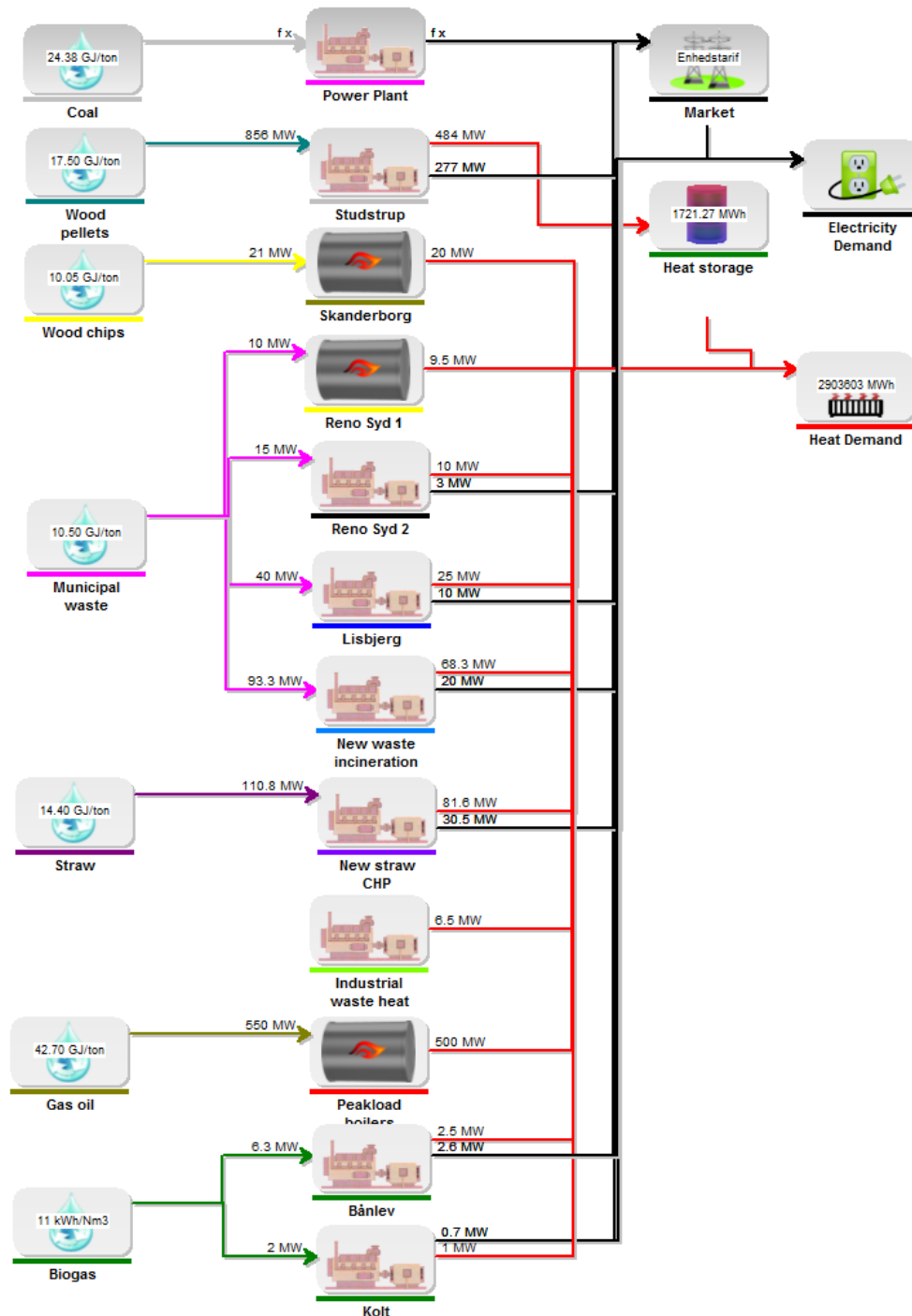
Figure 91: Reference system design for the Aarhus case study.
