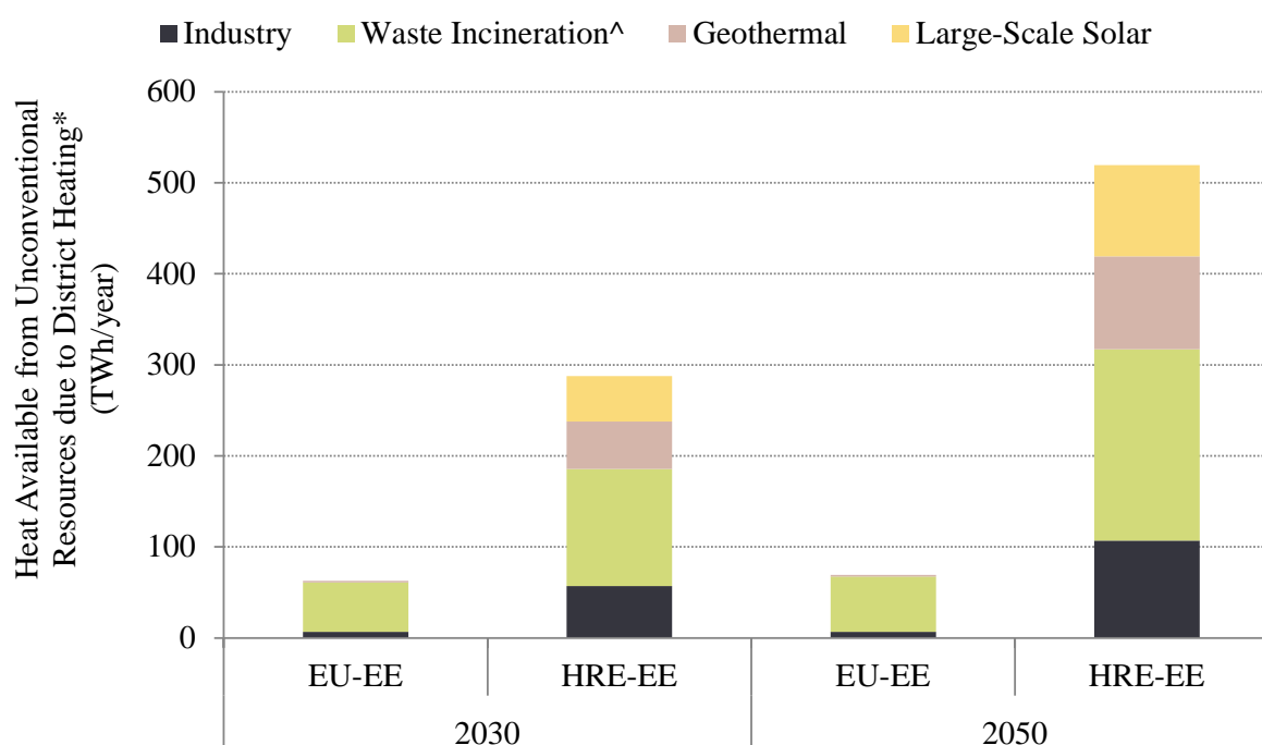
Figure 56: Heat from unconventional resources in the EU-EE and HRE-EE scenarios for the years 2030 and 2050.
