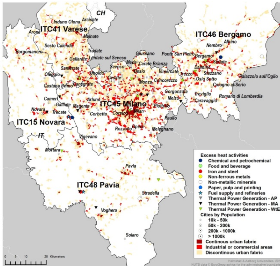
Figure 29: Example of Expansion NUTS3 region hot spots: large clusters of NUTS3 region excess heat hot spots in the Milan region in Italy.
