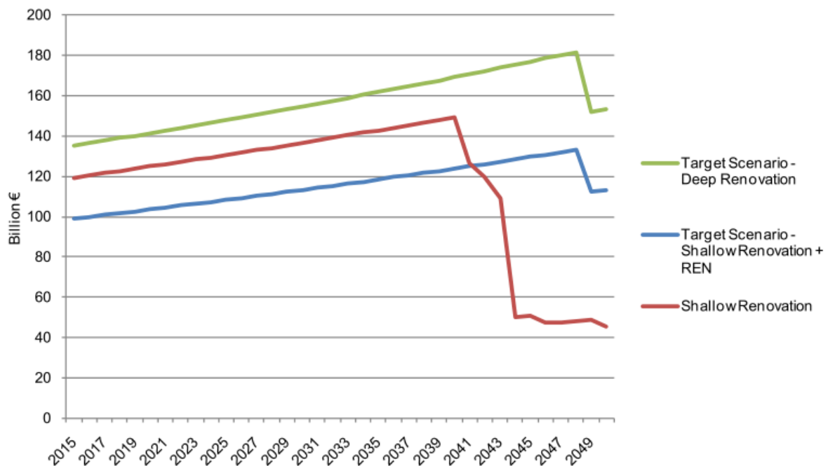
Figure 72: Annual investment costs for insulation and windows in the three scenarios created by Ecofys for energy efficiency in the EU27 [Boermans, Bettgenhäuser et al., 2012].
