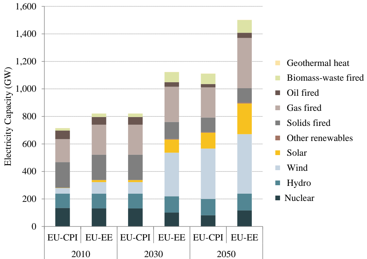
Figure 36: Electricity capacity by fuel in the EU-CPI scenario from the first pre-study [1] and the EU-EE scenario used in this study.
