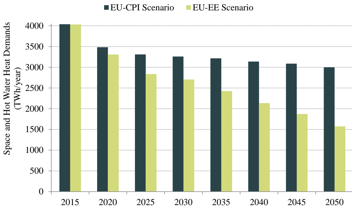
Figure 39: Total heat demand for the residential and services sectors in the EU-CPI scenario from the first pre-study [1] and EU-EE scenario used in this study for 2015-2050.
