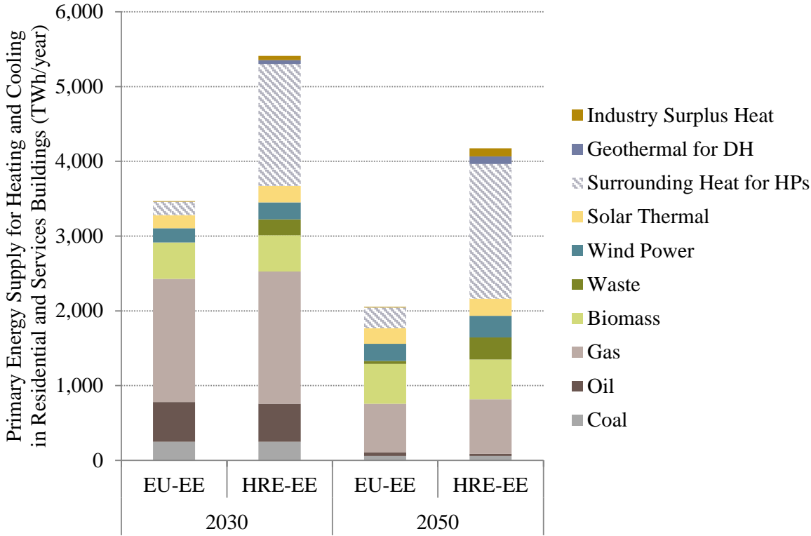
Figure 62: Primary energy supply for heating and cooling in residential and services buildings in the EU-EE and HRE-EE scenarios for the years 2030 and 2050.
