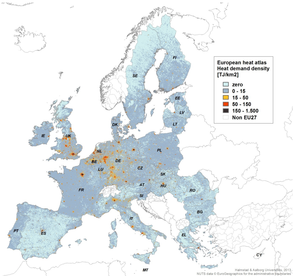
Figure 2: New European Heat Atlas developed in this study.
