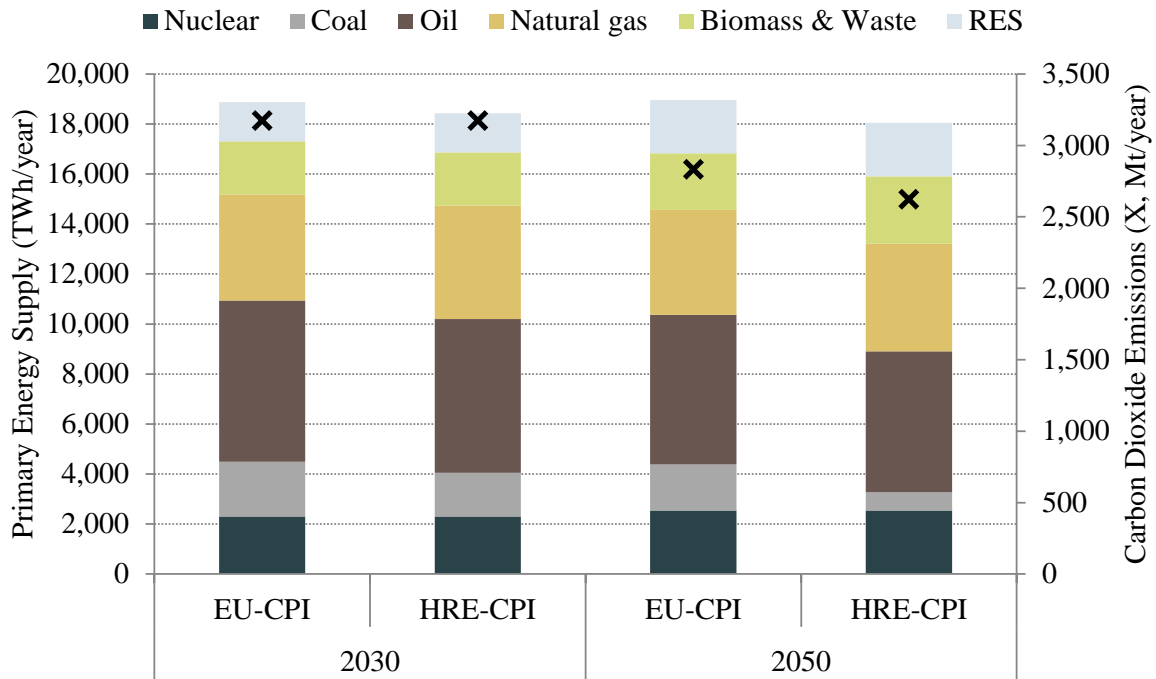
Figure 6, Primary energy supply and carbon dioxide emissions in the EU-CPI and HRE-CPI scenarios for the years 2030 and 2050.
