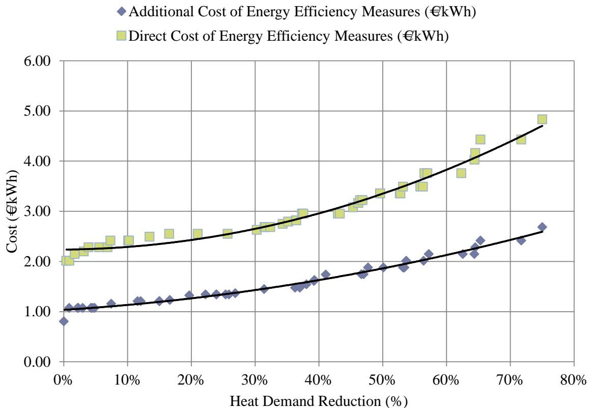
Figure 65: Additional and direct costs for energy efficiency measures that reduce the heat demand by different percentages based on Danish buildings (scenario C) [43].
