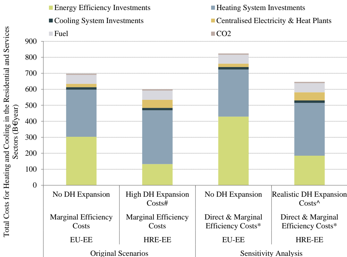
Figure 66: Total annual costs for heating and cooling in the residential and services sectors for the EU-EE and HRE-EE scenarios in 2050 for different energy efficiency and district heating cost assumptions. *Represents a scenario with 50% additional energy efficiency costs and 50% direct energy efficiency costs (see Figure 65). #Assumes that all additional district heating in the EU27 is in areas with a heat density less than 50 TJ/km 2 . ^Based on forecasted heat densities in the European Heat Atlas (Figure 14).
