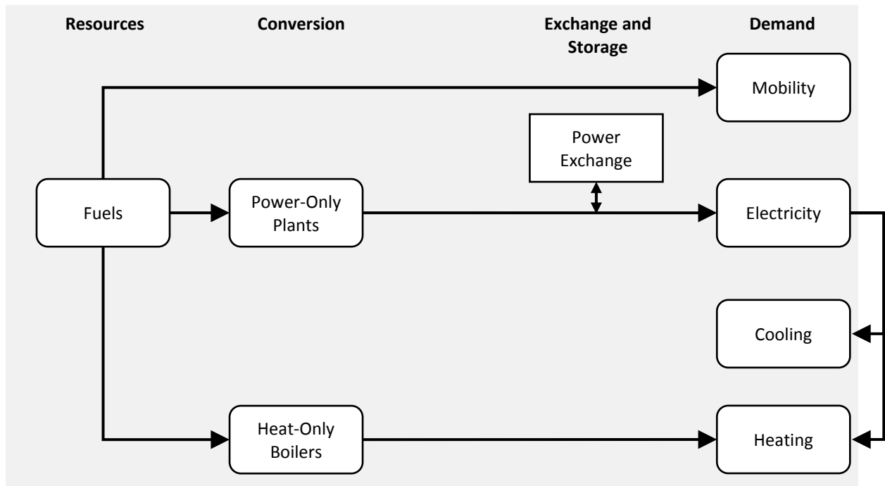
Figure 57: Interaction between sectors and technologies in segregated energy systems [51].
