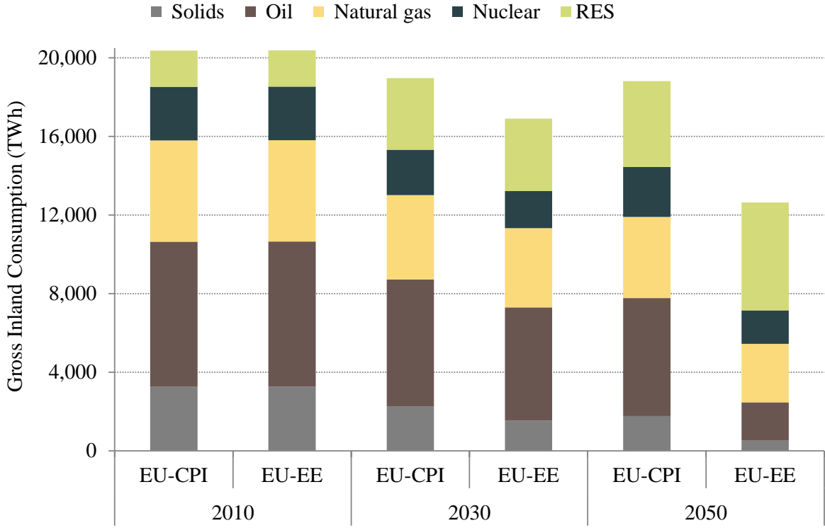
Figure 35: Gross inland consumption in the EU-CPI scenario from the first pre-study [1] and the EU-EE scenario used in this study. Note: electricity is excluded from this diagram since it only represents the net annual exchange which is less than 0.25% of the total in all years.
