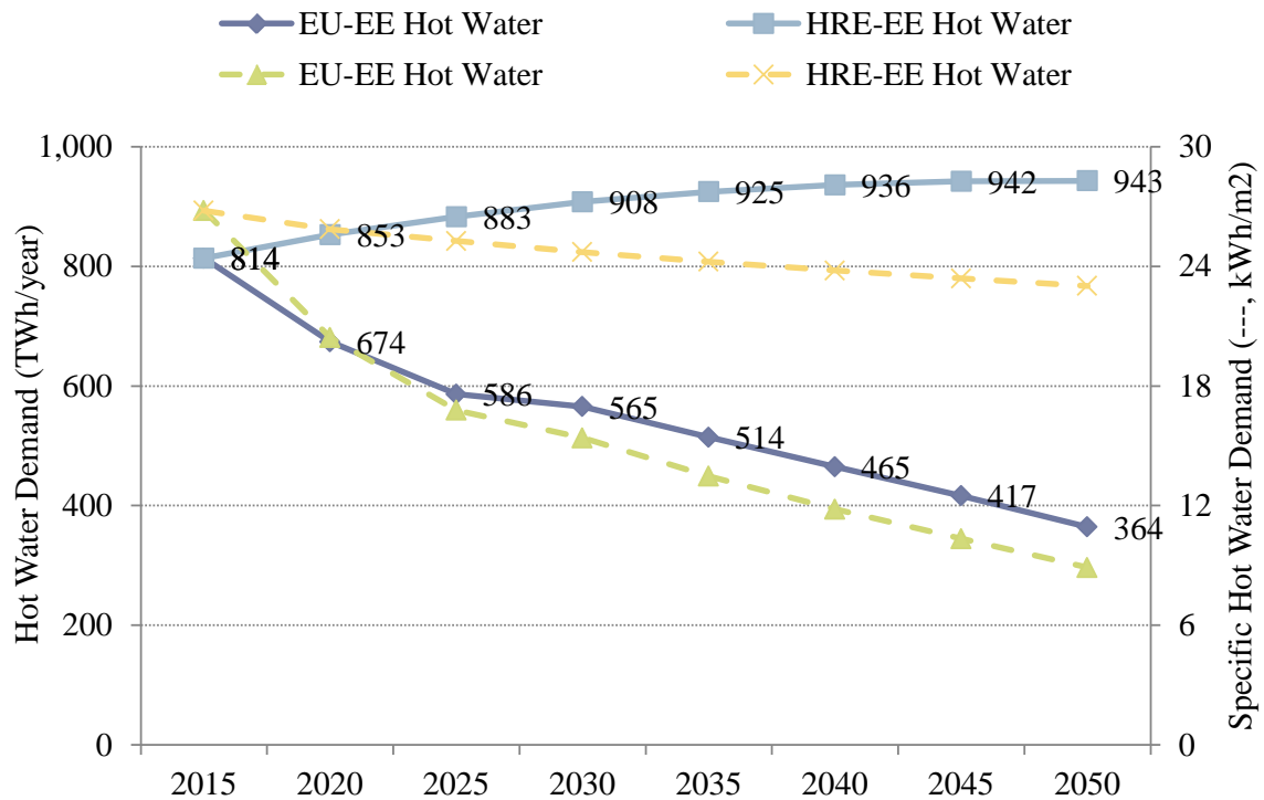
Figure 46: Original hot water demand in the EU-EE scenario and the new hot water demand for the HRE-EE scenario, along with the corresponding specific hot water demands (dotted lines).
