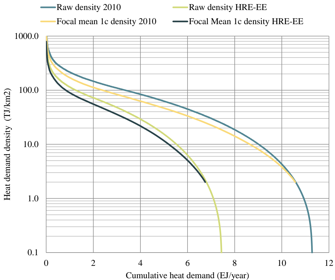
Figure 15: Cumulative heat demand according to the European Heat Atlas in 2010 and in the Heat Roadmap Europe Energy Efficiency (HRE-EE) scenario, by two different types of heat density calculations. Raw density is the density calculated in each square kilometre cell, while Focal mean density is the density if calculating the mean of a cell and its neighbourhood cells, thereby levelling out density values but resulting in more coherent prospective district heating areas.
