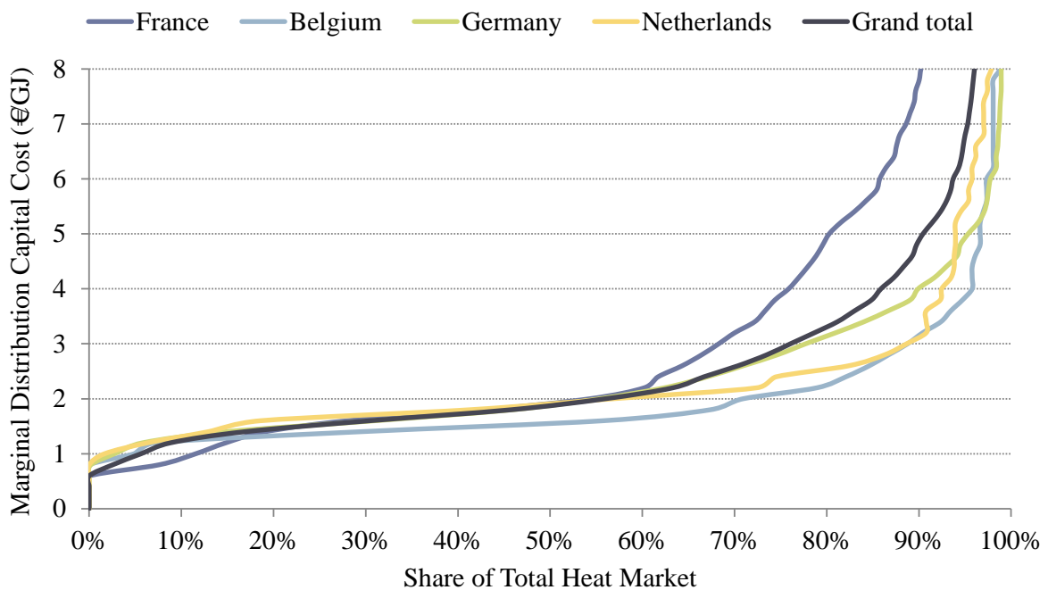
Figure 23: Current marginal distribution capital cost levels and corresponding urban district heating heat market shares in four studied European countries in 2008 [41].
