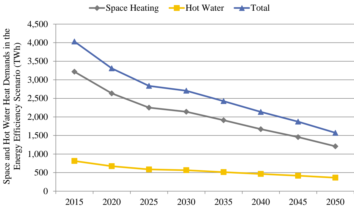
Figure 69: Space heating and hot water demand in the Energy Efficiency scenario between 2015 and 2050.
