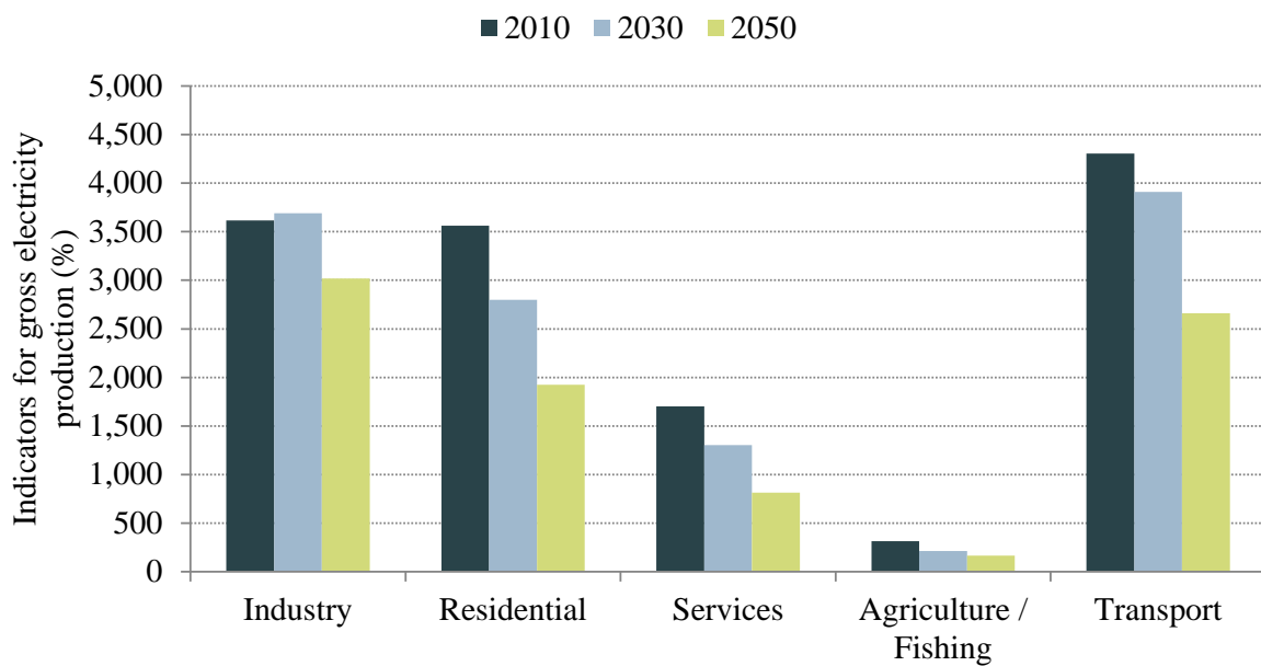
Figure 38: Final energy consumption by sector in the EU-EE scenario for the years 2010, 2030, and 2050.
