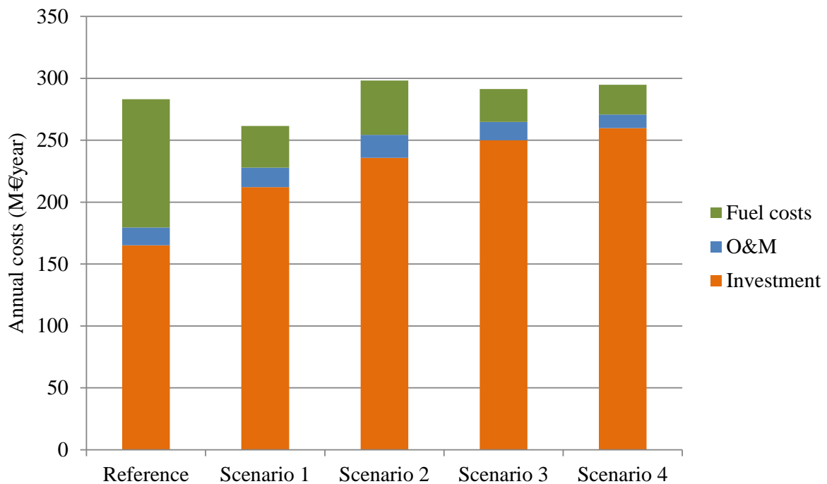
Figure 99: Annualised costs for all scenarios, categorised by fuel, O&M and investment costs
