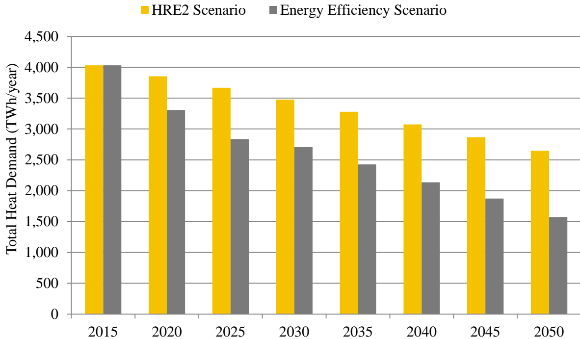
Figure 78: Total heat demand for the new scenario assumed in this study and the EE scenario for 2015-2050.
