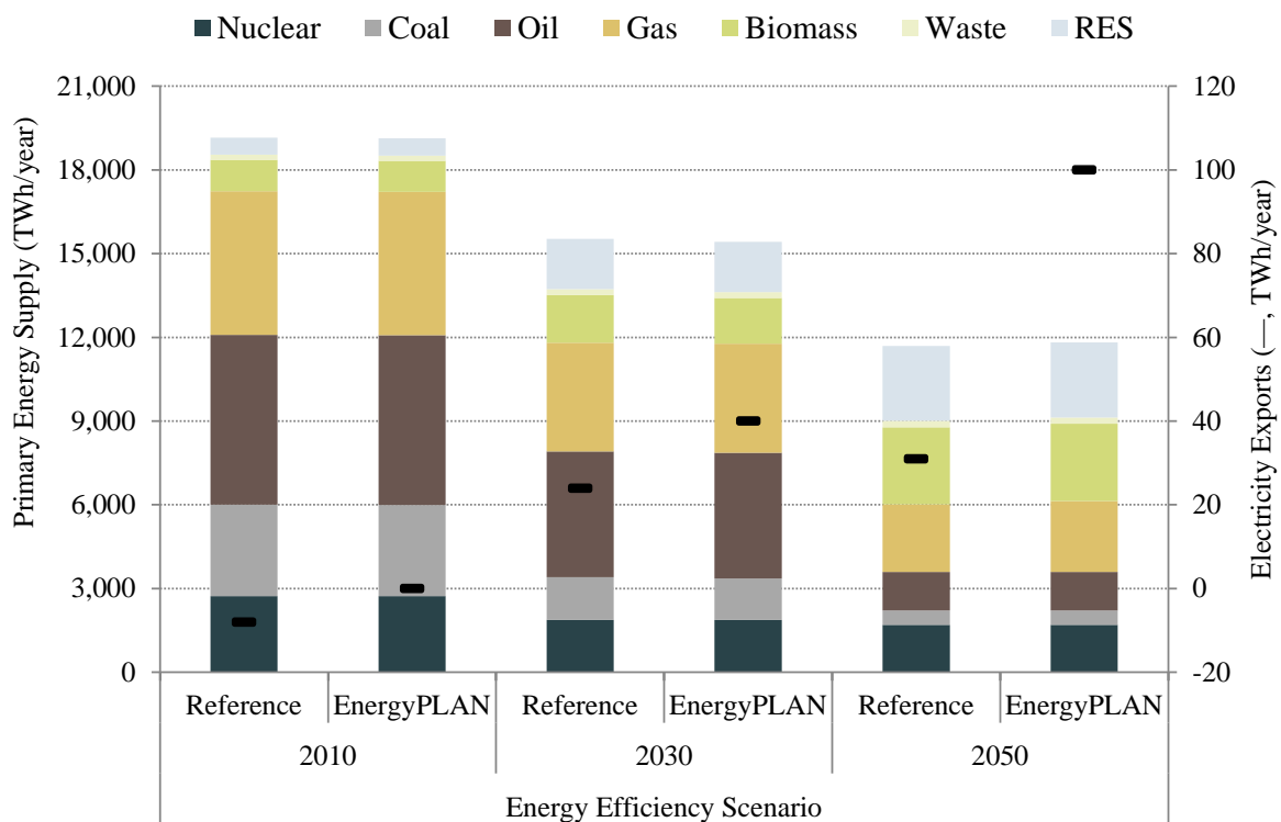
Figure 43: Primary energy supply by fuel and the net electricity exports for the EU-EE scenario from the original 'reference' projections and the EnergyPLAN model.
