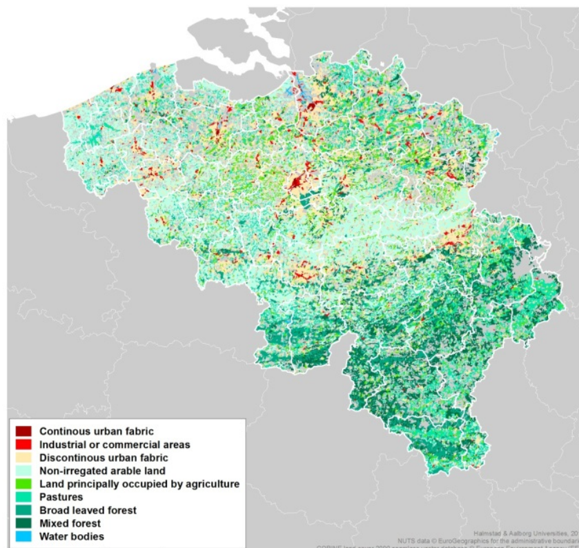
Figure 17: Example of land cover data labels for Belgium from the European CORINE land cover 2000 seamless vector database [28].
