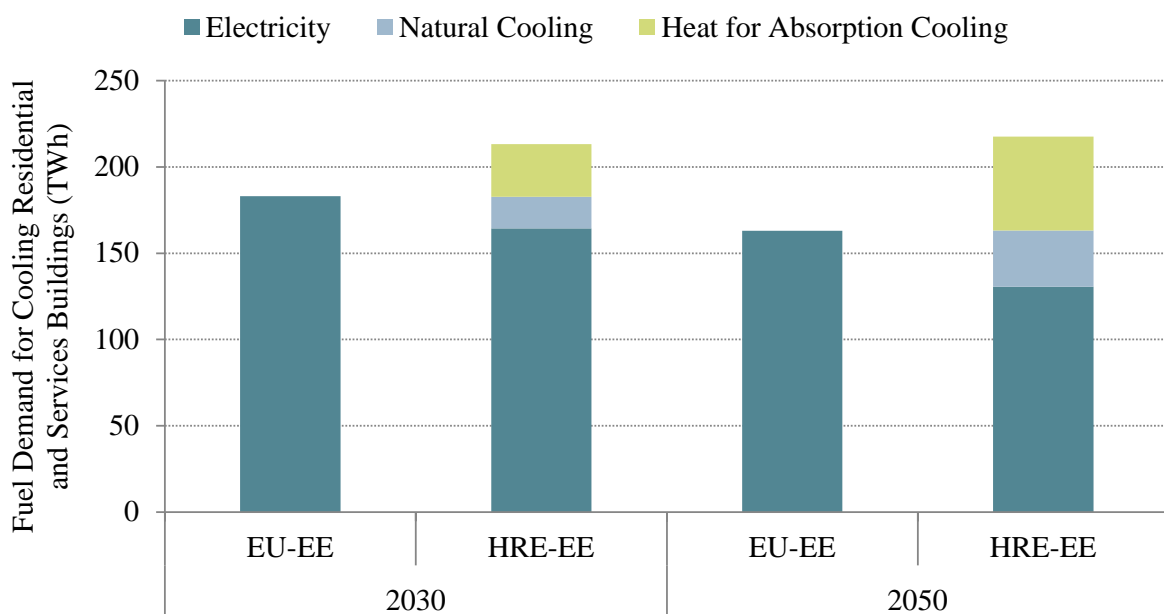
Figure 54: Fuel demand for cooling residential and services buildings in the EU-EE and HRE-EE scenarios for the years 2030 and 2050.
