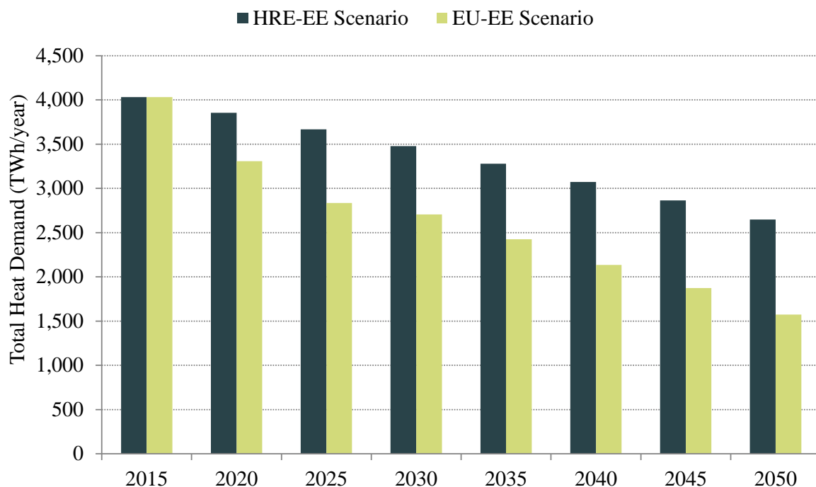
Figure 48: Total heat demand for the EU-EE and HRE-EE scenarios for 2015-2050.
