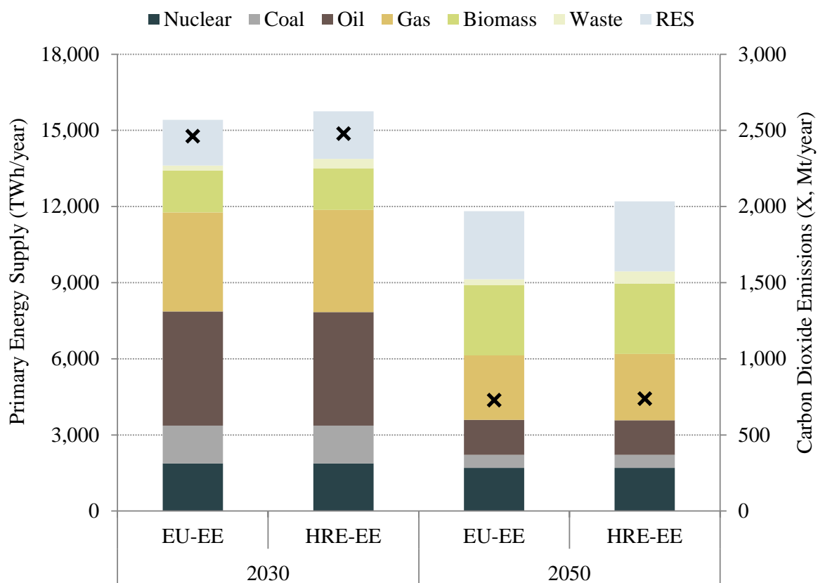
Figure 61: Primary energy supply and carbon dioxide emissions for the EU-EE and HRE-EE scenarios in the years 2030 and 2050.
