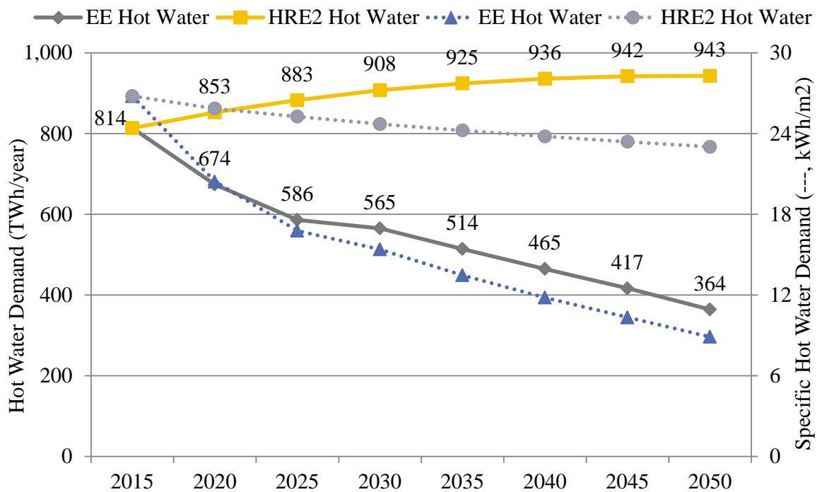
Figure 76: Original hot water demand in the EE scenario and the new hot water demand which is used in this study, along with the corresponding specific hot water demands (dotted lines).
