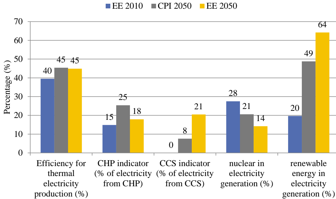
Figure 87: Indicators for gross electricity production in the EU-CPI scenario from the first pre-study [1] and the EU-EE scenario used in this study.
