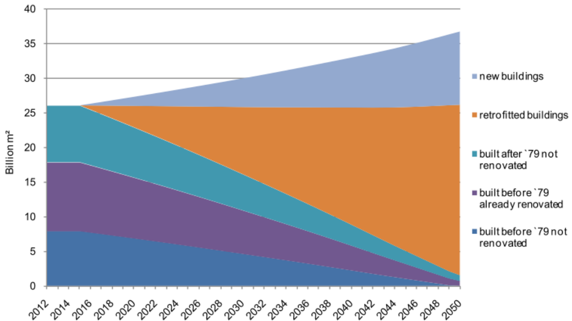
Figure 67: Heated floor area EU27 – track “Target Scenario, Deep Renovation” [billion m²]
