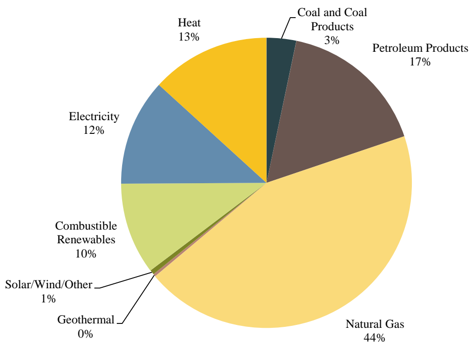
Figure 8: Composition of the origin for heat supply to residential and service sector buildings in EU27 during 2010. Total heat supply was 11.8 EJ (3300 TWh), not including indirect heat supply from all indoor electricity use. Labels refer to the standard commodity groups used in the IEA energy balances. Heat denotes mainly heat from district heating systems. Data sources: IEA energy balances for 2010 complemented with some external estimations.
