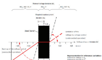
Fig. 2. Reactive output current during disturbances [1]
