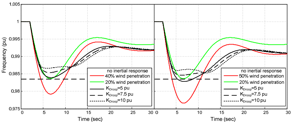
Fig. 4.50. System frequency for different K_{Droop} values where T_{Droop}=9s , H_{WPP}=5pu , T_{WPP}=0.025s , and R_{WPP}=1pu/s
