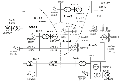
Fig. 1. Generic 12-bus test system [20]
