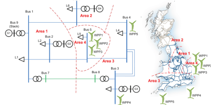
Fig. 5. Wind penetration scenarios for generic 12-bus system.
