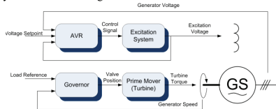
Fig. 6. Structure of conventional power plant model.
