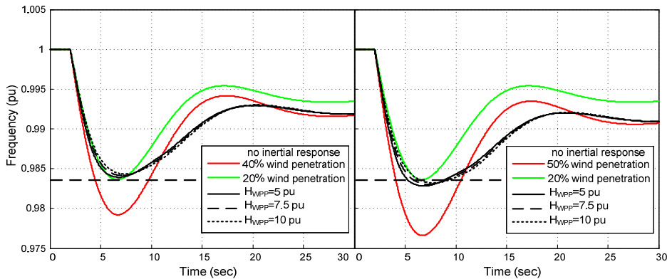
Fig. 4.44. System frequency for different H_{WPP} values where R_{WPP}=1 pu/s, T_{WPP}=0.025 s, K_{Droop}=5 pu, and T_{Droop}=9 s for 40% and 50% wind power penetration scenarios. ROCOF is given in Fig. 4.45 for 200ms following the disturbance. It can be noticed that during this time, ROCOF has been changed and come close to the CPP inertial
