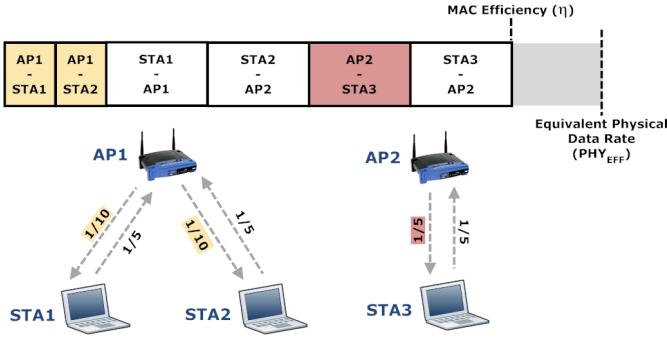
Fig. 1: An illustration of the resource partitioning predicted by the model. Two neighboring co-channel cells displayed.
