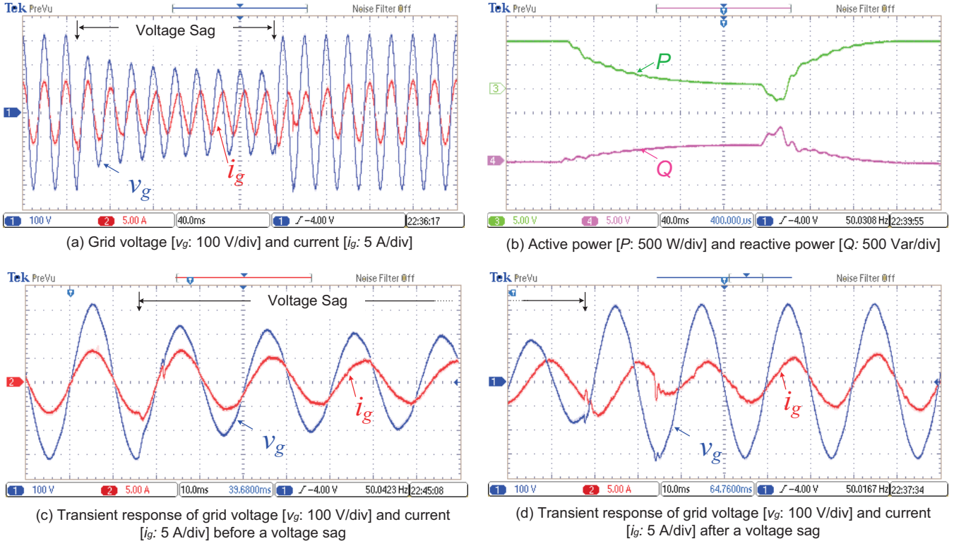
Fig. 16. Experimental results of a single-phase grid-connected system under voltage sag (0.45 p.u.) using PR controller and SOGI-OSG PLL synchronization method, [ t = 40 \text{ ms/div} ].
