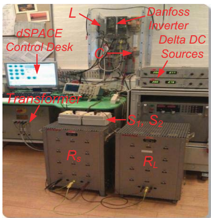
Fig. 12. Experimental setup.
