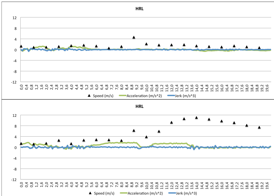
Figure 11. Two examples of significant changes in speed without significant effect on the acceleration pattern due to poor GPS connection in densely built-up areas.
