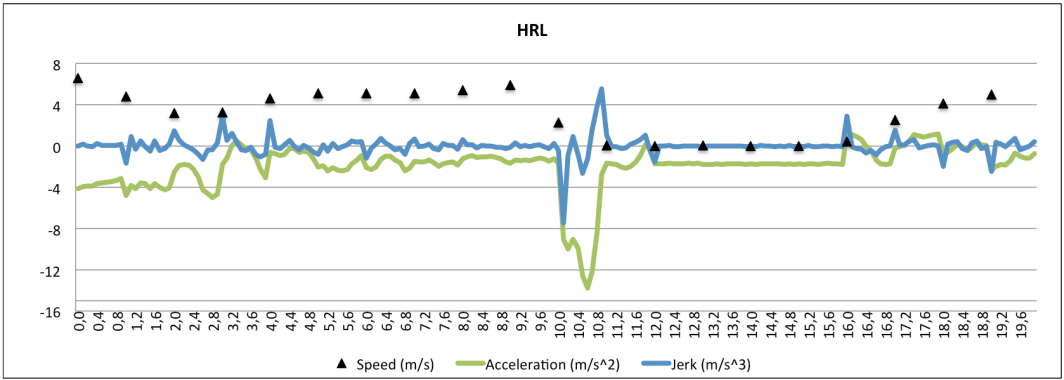
Figure 7. Significant jerk and clear speed reduction.
