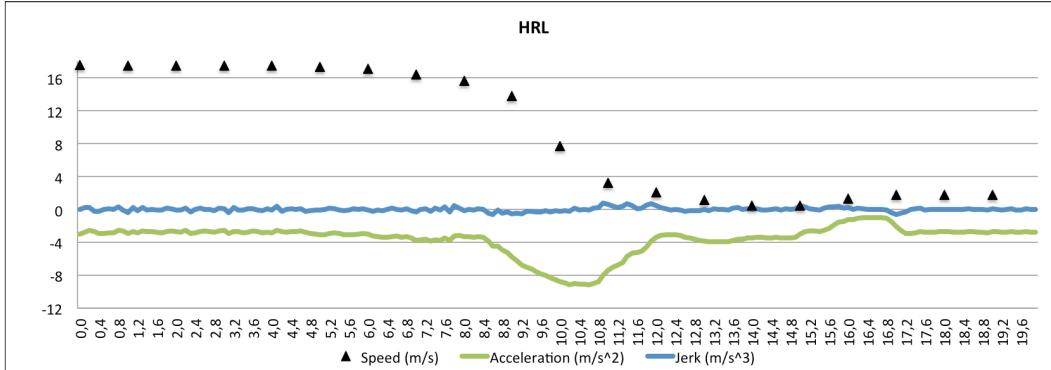
Figure 10. Significantly reduced speed without clear jerks.
