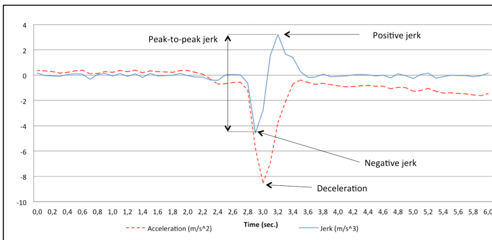
Figure 4: Peak-to-peak jerk, in case of typical braking procedure and during a conflict.
