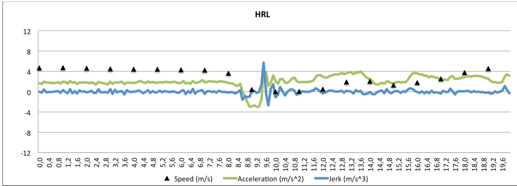
Figure 9. Significant jerk at low-speed approaching.
