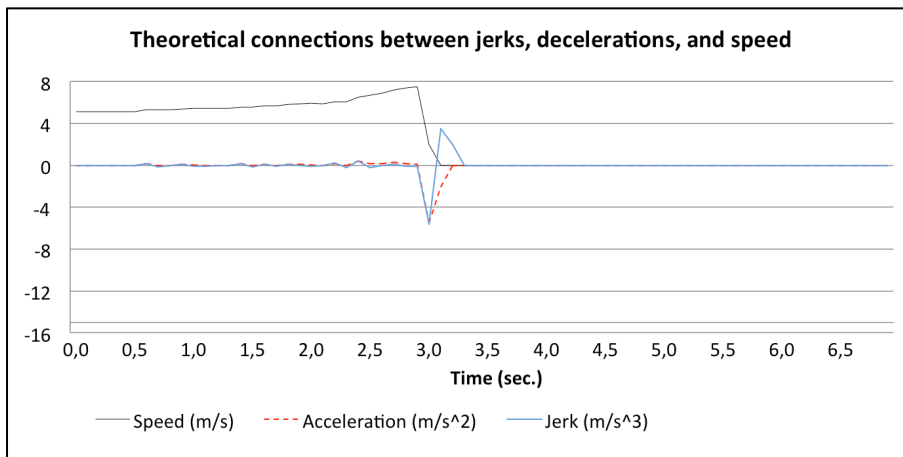
Figure 2 Theoretical connections between jerks ( m/s^3 ), decelerations ( m/s^2 ), and speed ( m/s ).
