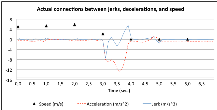
Figure 3: Speed, accelerations and jerks and their interconnections in practice.
