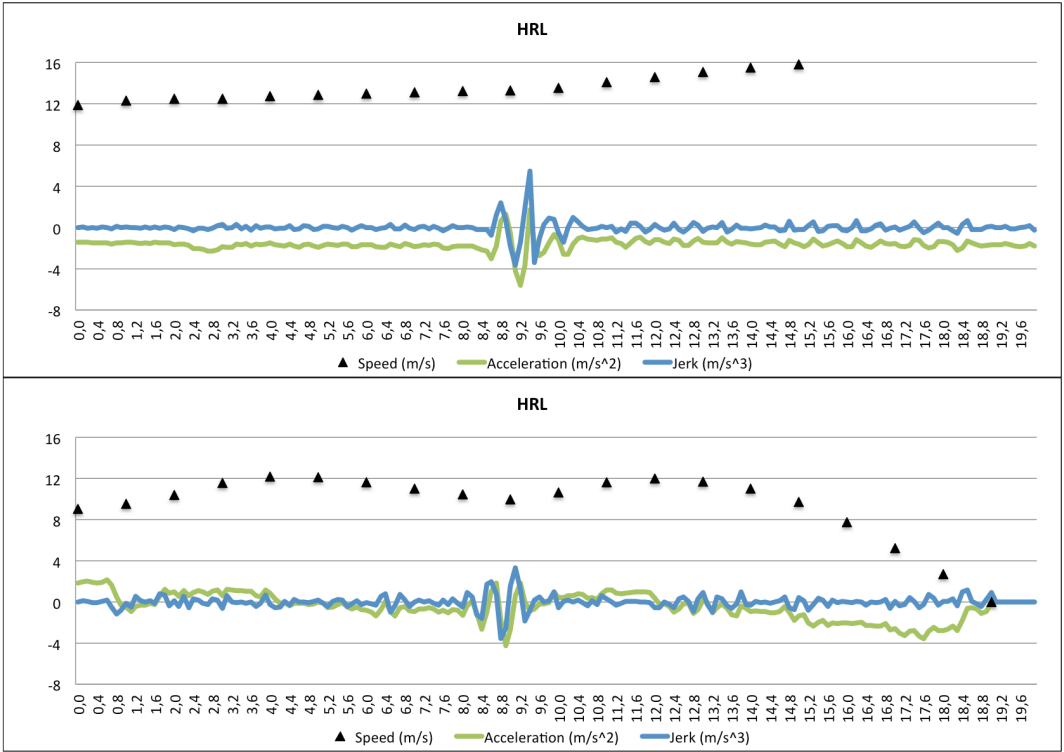
Figure 8. Two examples of significant decelerations and jerks with no connection to change in speed.
