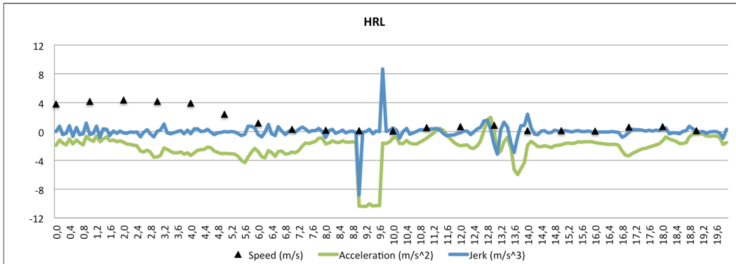
Figure 5. A reduced speed followed by a significant deceleration with abrupt ending. X-axis is sequential time (sec.). The Y-axis is m/s., m/s 2 , and m/s 3 .
