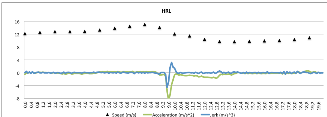
Figure 6. Significant although short deceleration.
