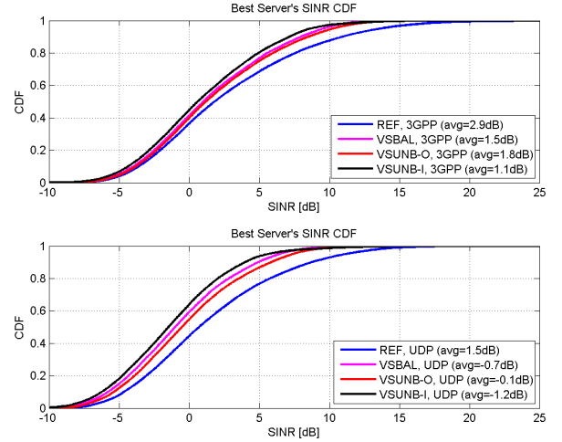
Fig. 3. SINR CDF of the 3x1REF and VS scenarios for (a) 3GPP model and (b) UDP Model.
