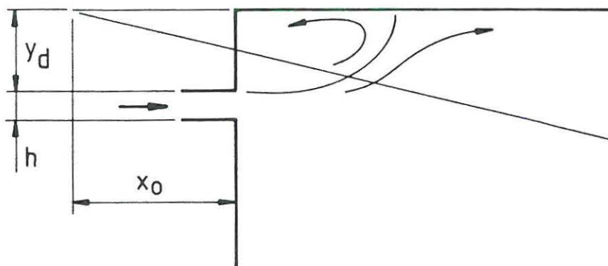
Fig. 2 Geometry of a linear slot diffuser placed at a distance from the ceiling.
