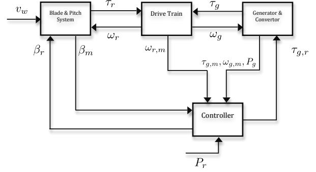
Fig. 1. Block diagram of the wind turbine model
