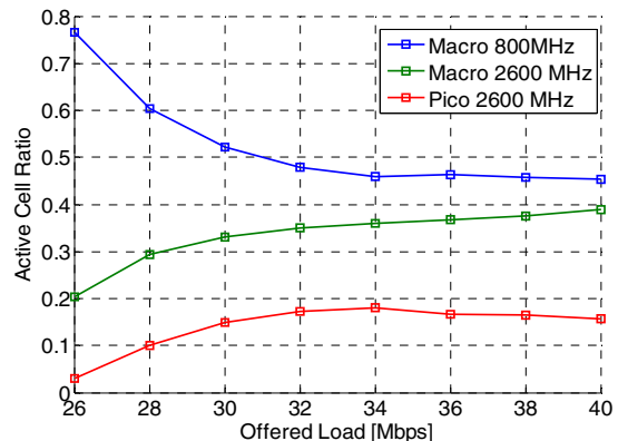
Figure 3: Distribution of Active Cells versus Offered Load
