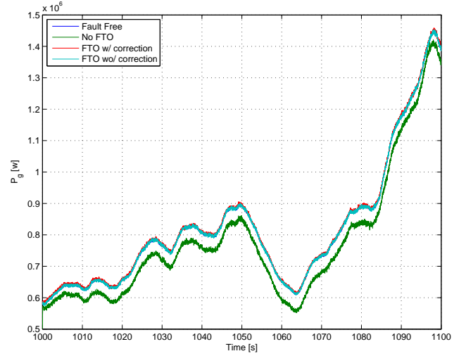
Fig. 7. P_g in the time period in which Fault # 3 is present. The controller is based on the estimated \omega_g . The plot shows the fault free case, as well as three cases with faults: one without any fault accommodation, the FT observer with and without the correction component.
