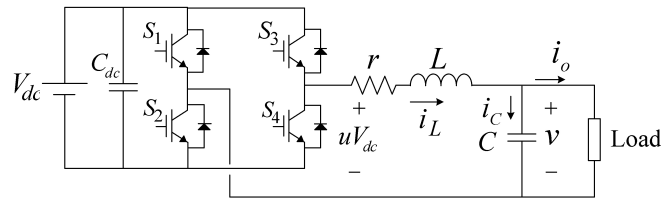
Fig. 1. Power stage of a single-phase VSI.
