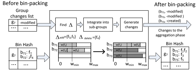
Fig. 6. Flow of data in the bin packing phase
