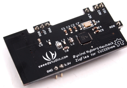
Figure 3. the ZigFlea add-on for the CUI32, developed by Øyvind Nyborg Hauback at the University of Oslo, Norway, sold by www.seeedstudio.com
