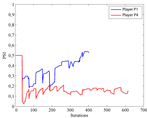
Fig. 10: Illustration of how database evolves. The figure shows the average PSI for all cases for player P1 and P4 as a function of the revision of the database.
