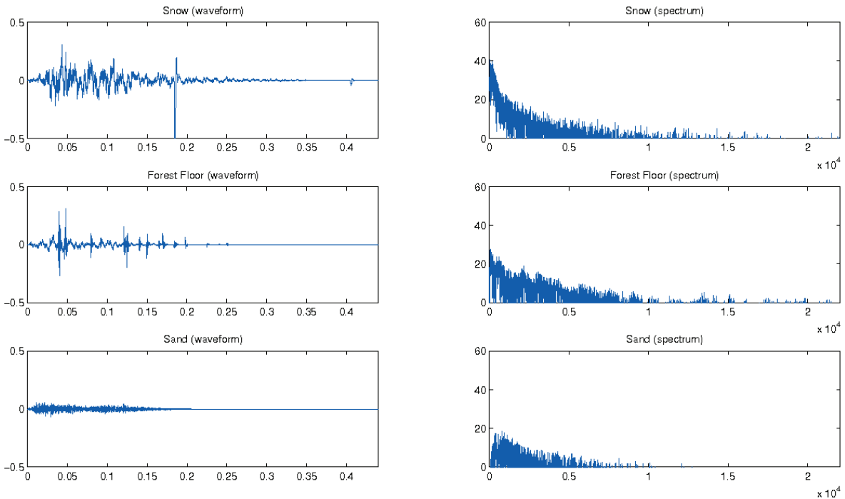
Fig. 3. Typical waveforms (left) and spectra (right) of the three simulated materials. The duration of the waveforms is expressed in milliseconds, the magnitude of the spectra in decibel.
