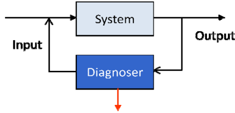
Figure 1.9: Active fault diagnosis diagram.
