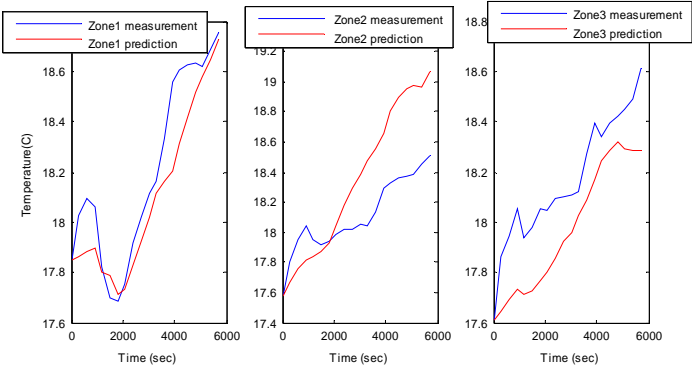
Figure 6.8: Indoor temperature for every zone.
