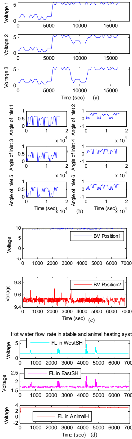
Figure 6.4: (a) voltage of fan, (b) the angle of inlets, (c) Ball-valve position for animal and stable heating systems, (d) Hot water flow rate in stable and animal heating systems.
