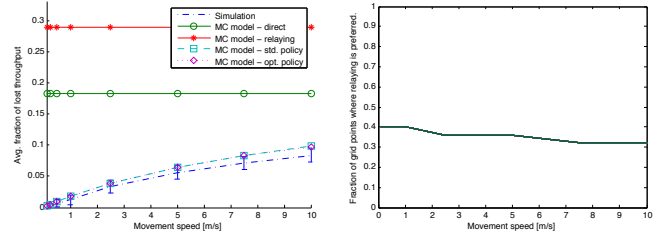
(a) Lost throughput
