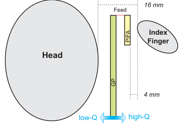
Fig. 2. Simulation set-up.
