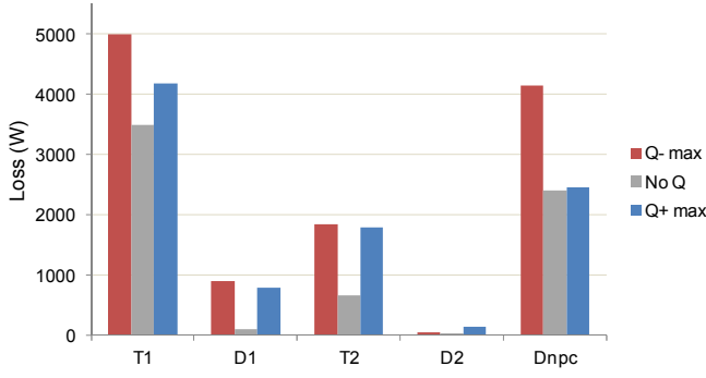
Fig. 16. Loss distribution of 3L-NPC inverter with different extreme reactive powers (Considering parallel converters).
