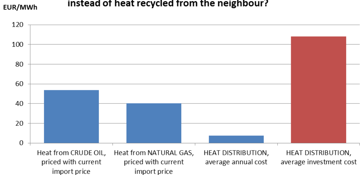
Figure 23: The simple socio-economic comparison between current import prices of fossil fuels and the heat distribution cost for connecting heat surpluses with heat demands. Current import price of crude oil has been set to 110 US$ per barrel.
